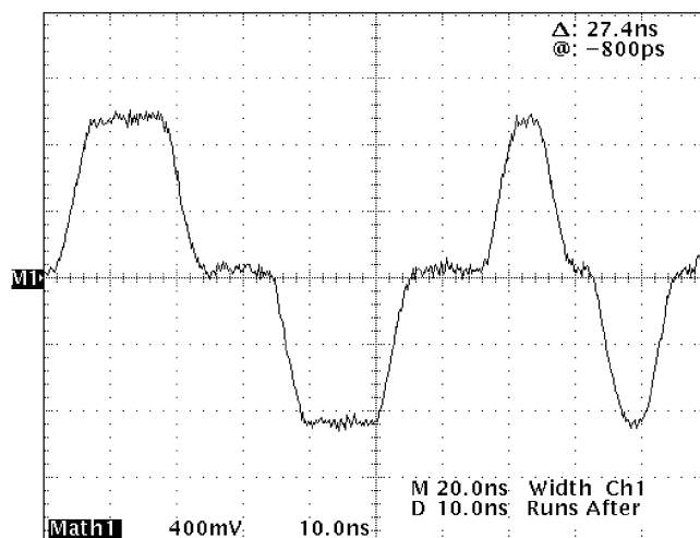
Figure 2. 100Mb Waveform
