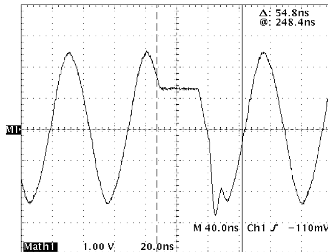
Figure 1. 10Mb Waveform
