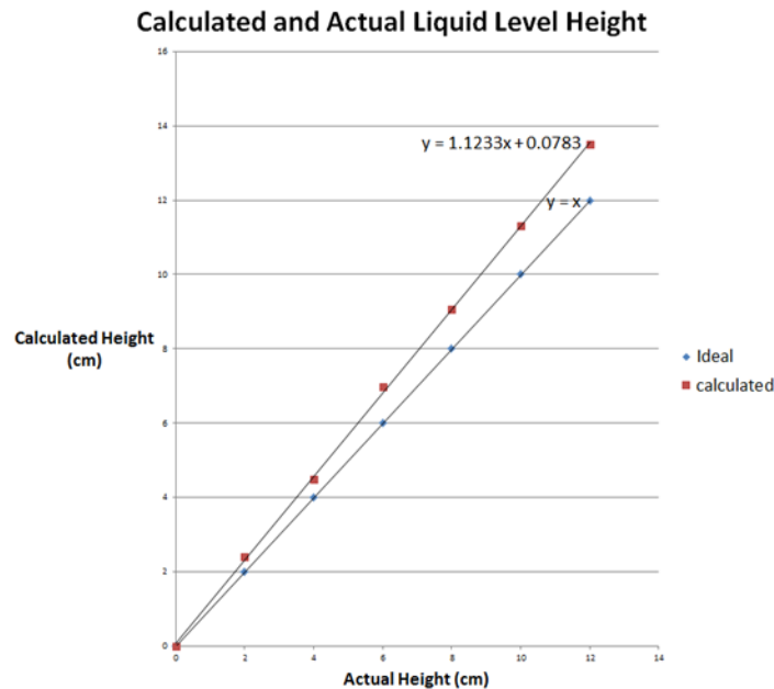
Figure 2. Calculated and Actual Liquid Level Height
