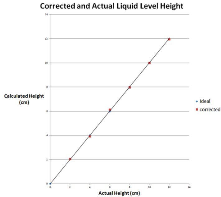
Figure 3. Corrected and Actual Liquid Level Height
