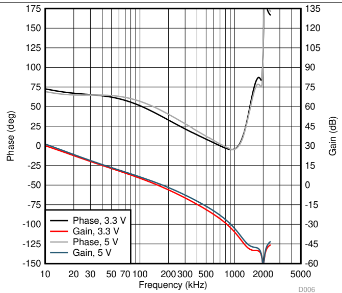
Figure 8. V_{\text{OUT}}=1000\text{ mV} , C_{\text{POL}}=44\ \mu\text{F}/\text{phase} , 2-phase configuration
