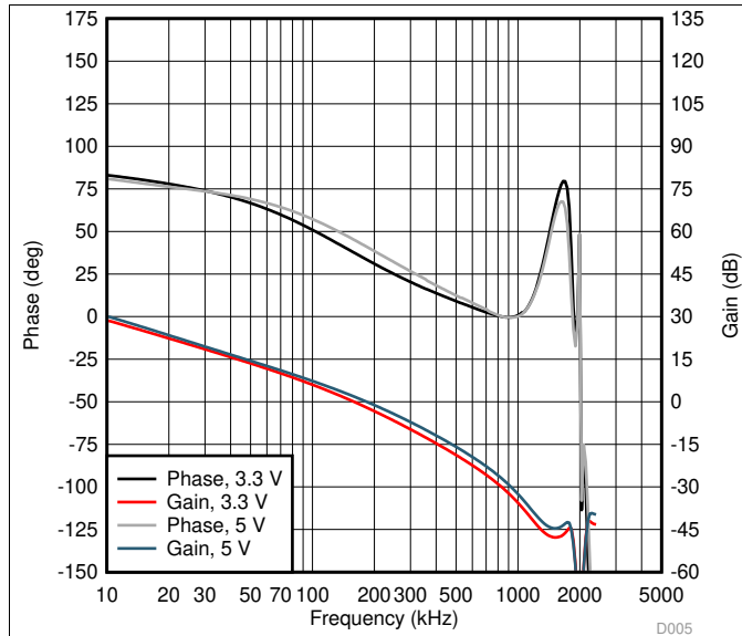
Figure 7. V_{\text{OUT}}=1000\text{ mV} , C_{\text{POL}}=44\ \mu\text{F}/\text{phase} , 1-phase configuration
