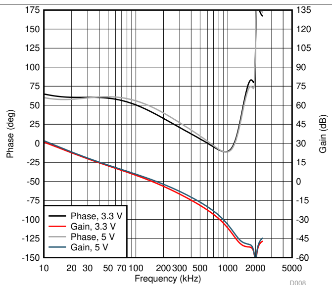
Figure 10. V_{\text{OUT}}=1000\text{ mV} , C_{\text{POL}}=44\ \mu\text{F}/\text{phase} , 4-phase configuration
