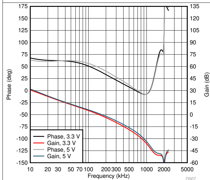
Figure 9. V_{\text{OUT}}=1000\text{ mV} , C_{\text{POL}}=44\ \mu\text{F}/\text{phase} , 3-phase configuration
