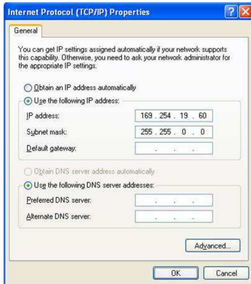
Figure 1. TCP/IP Properties
