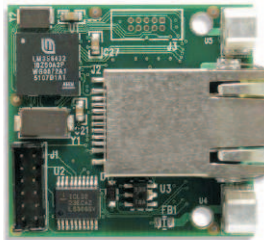
Figure 2. Stellaris Serial to Ethernet Module
