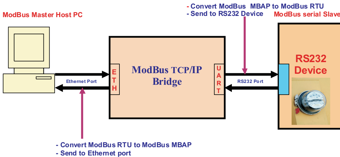
Figure 1. Stellaris Serial to Ethernet Block Diagram
