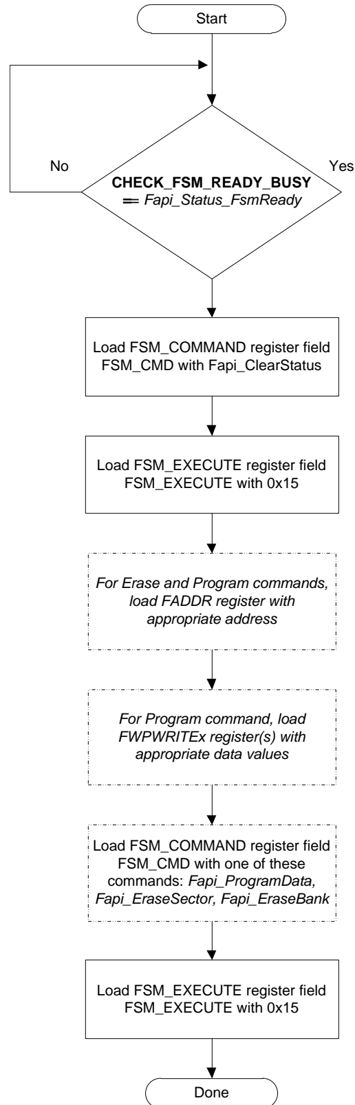
Figure 15. Recommended Command Execution Flow
