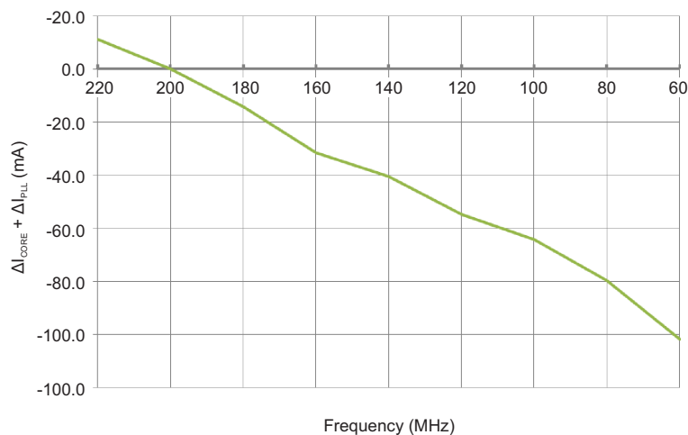
Figure 3. Current Reduction Versus HCLK on RM48L950
