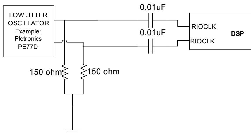
Figure 4. RIOCLK Multiple Devices LVDS Clock Solution
