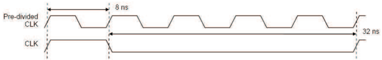
Figure 14. VLYNQ Clock Divider Example
