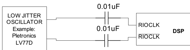
Figure 3. RIOCLK Single Device LVDS Clock Solution
