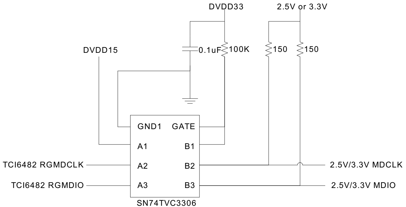
Figure 13. HSTL to LVCMOS Translation
