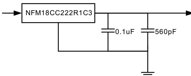
Figure 8. Recommended Power Supply Filter
