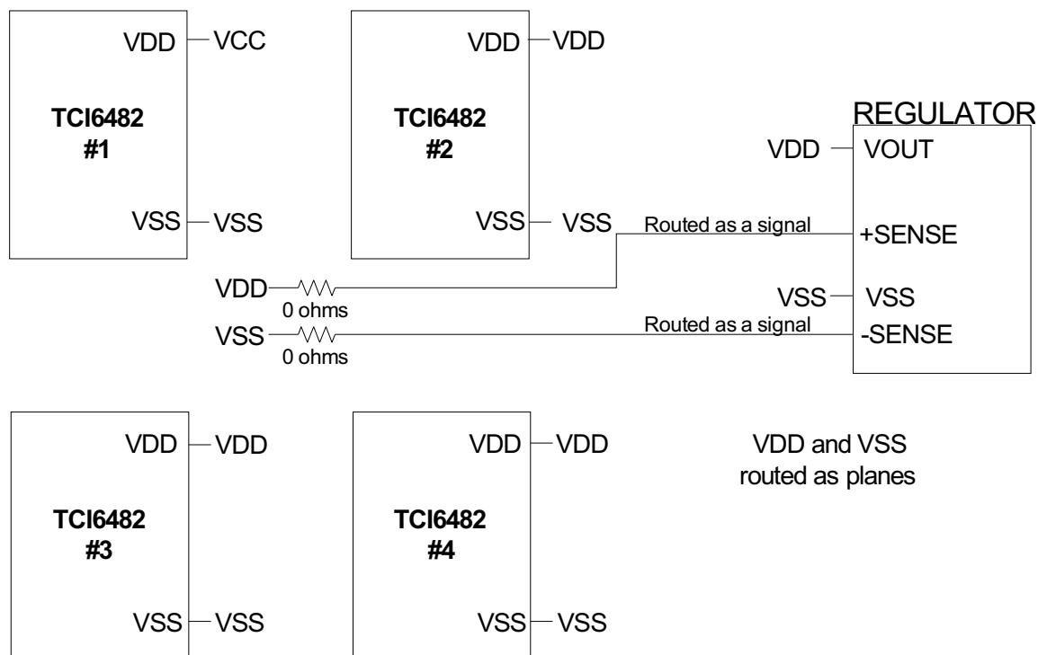
Figure 10. Multiple DSP Remote Sense Connections
