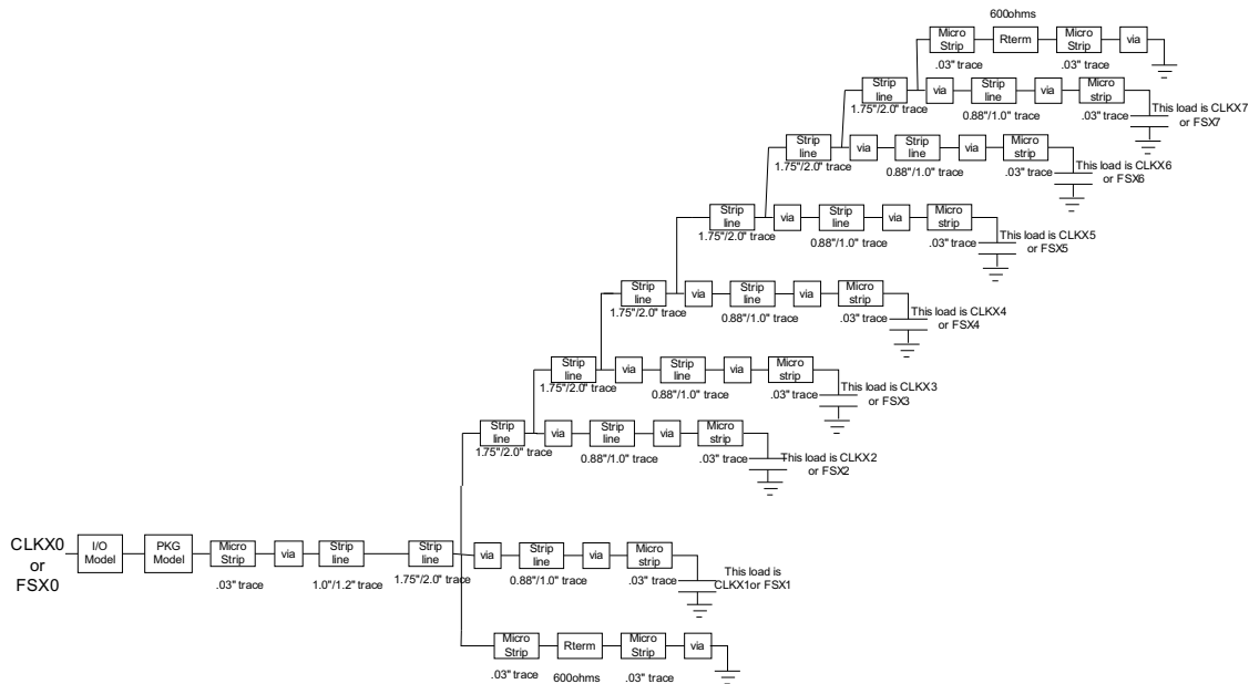
Figure 12. McBSP 8 Load Routing Topology
