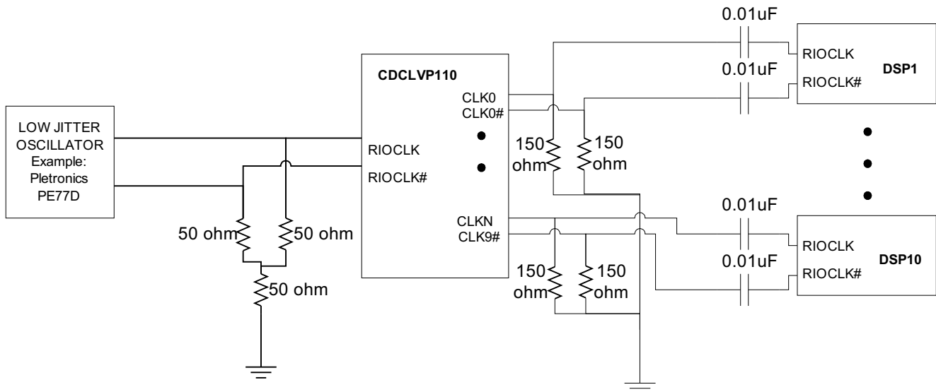
Figure 6. RIOCLK Multiple Devices LVPECL Clock Solution
