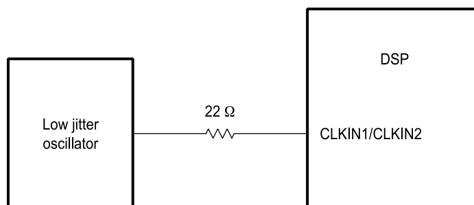
Figure 1. CLKIN1, CLKIN2 Single Device Clock Solution
