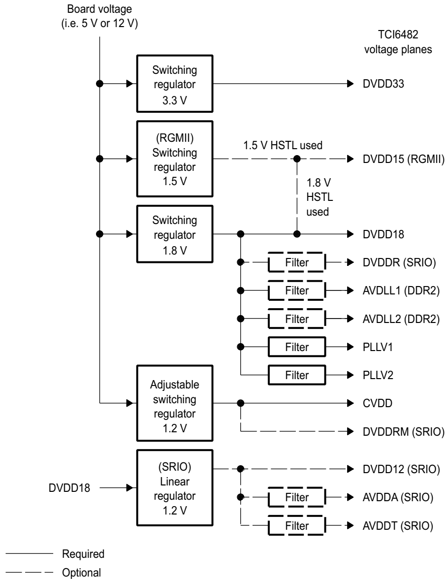
Figure 7. Power Supply Generation
