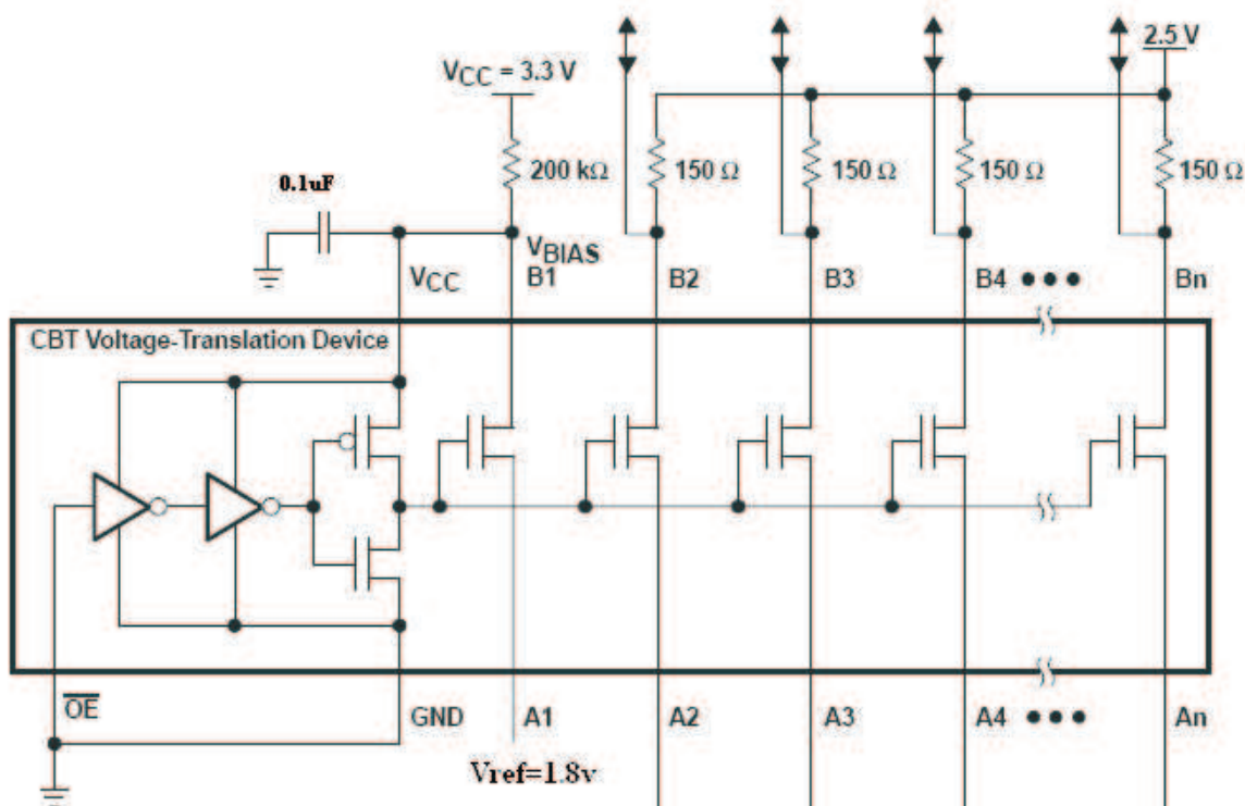
Figure A-1. RGMII Voltage Level Translation Circuit
