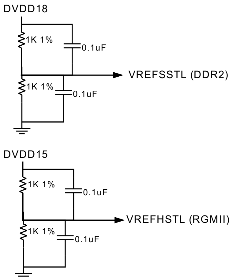
Figure 9. Reference Voltage Generation
