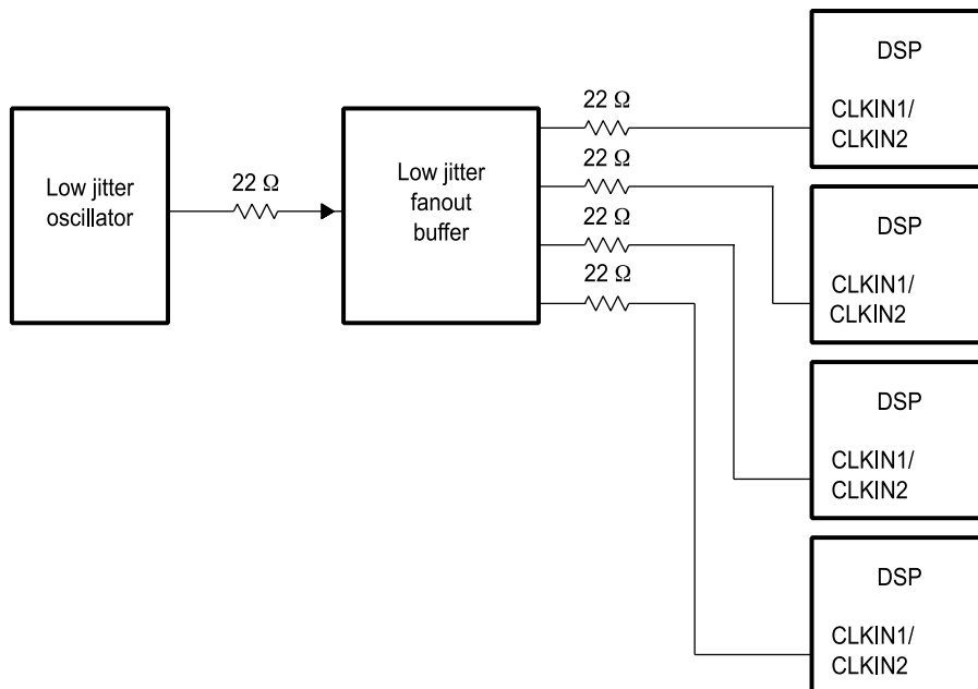
Figure 2. PLL1, PLL2 Multiple Device Clock Solution
