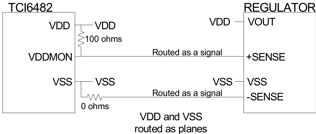
Figure 11. Single DSP Remote Sense Connections
