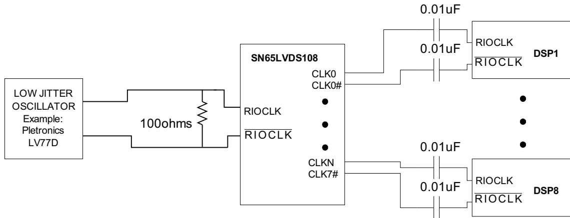
Figure 5. RIOCLK Multiple Devices LVDS Clock Solution
