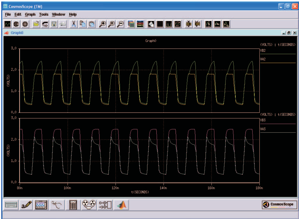
Figure A-3. 125MHz Signal from A2 to B2 and From B3 to A3
