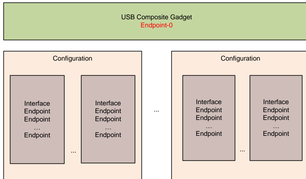
Figure 1. Block Diagram of USB Composite Gadget
