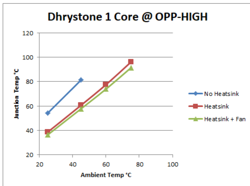
Figure 7. Dyrystone (Core 1) at OPP_HIGH (Junction Temp vs Ambient Temp)
