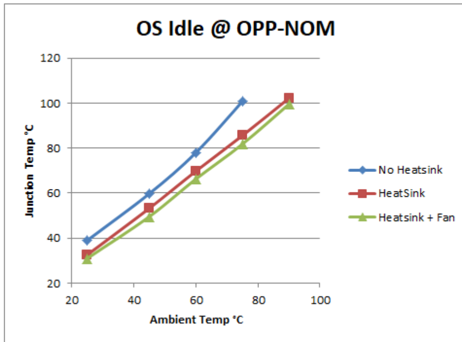
Figure 1. OS Idle - OPP_NOM (Junction Temp vs Ambient Temp)
