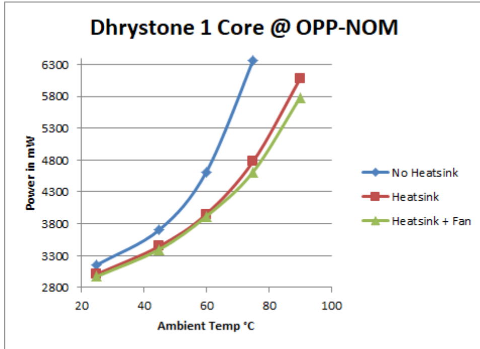
Figure 4. Dhrystone (Core 1) at OPP_NOM (Power Consumption vs Ambient Temp)
