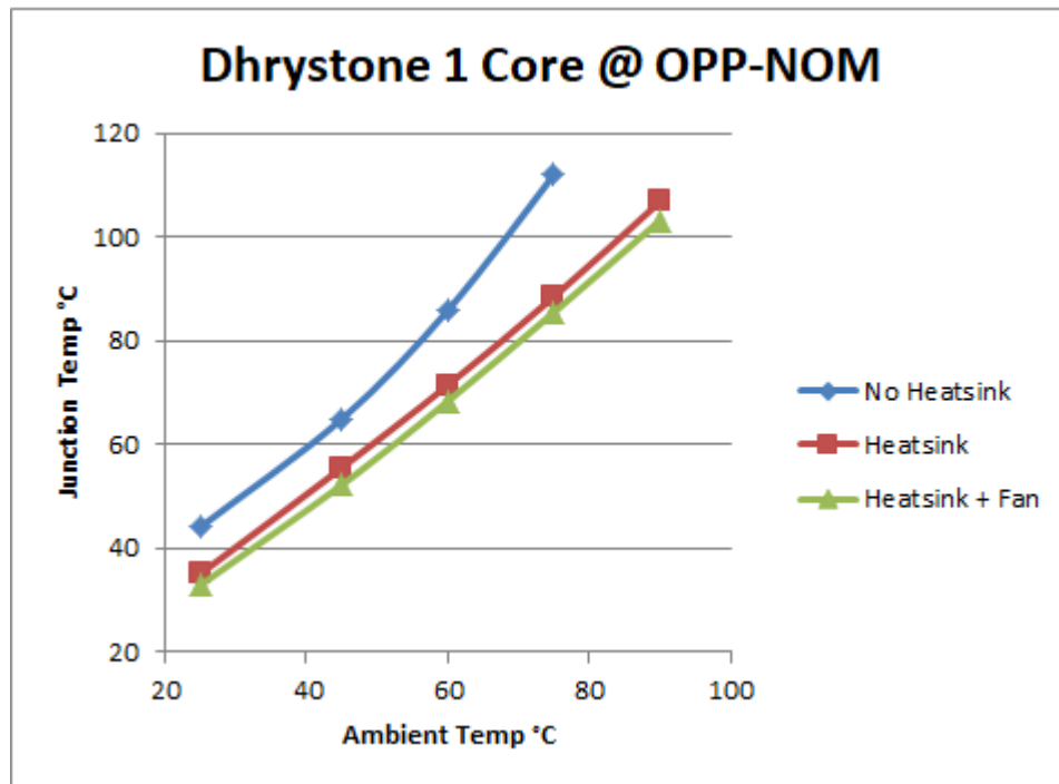
Figure 3. Dyrystone (Core 1) at OPP_NOM (Junction Temp vs Ambient Temp)
