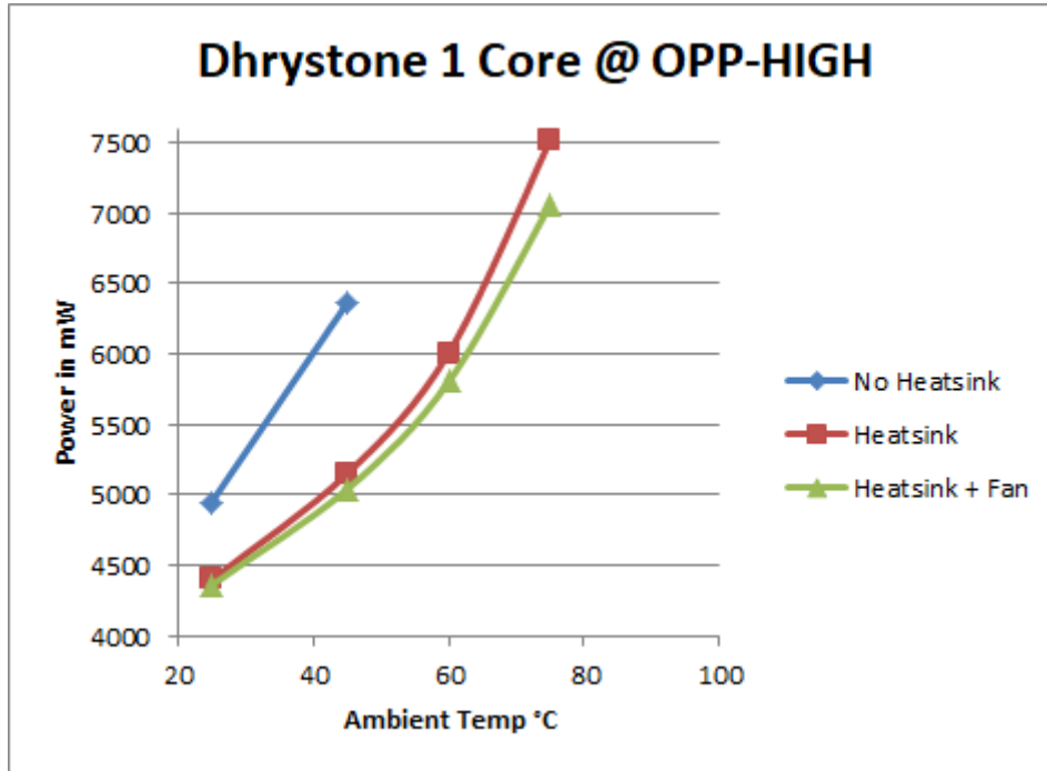
Figure 8. Dyrystone (Core 1) at OPP_HIGH (Power Consumption vs Ambient Temp)
