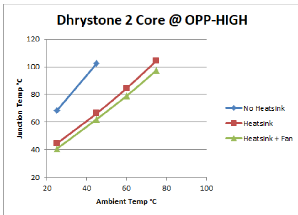
Figure 9. Dyrystone (Core 1 & Core 2) at OPP_HIGH (Junction Temp vs Ambient Temp)
