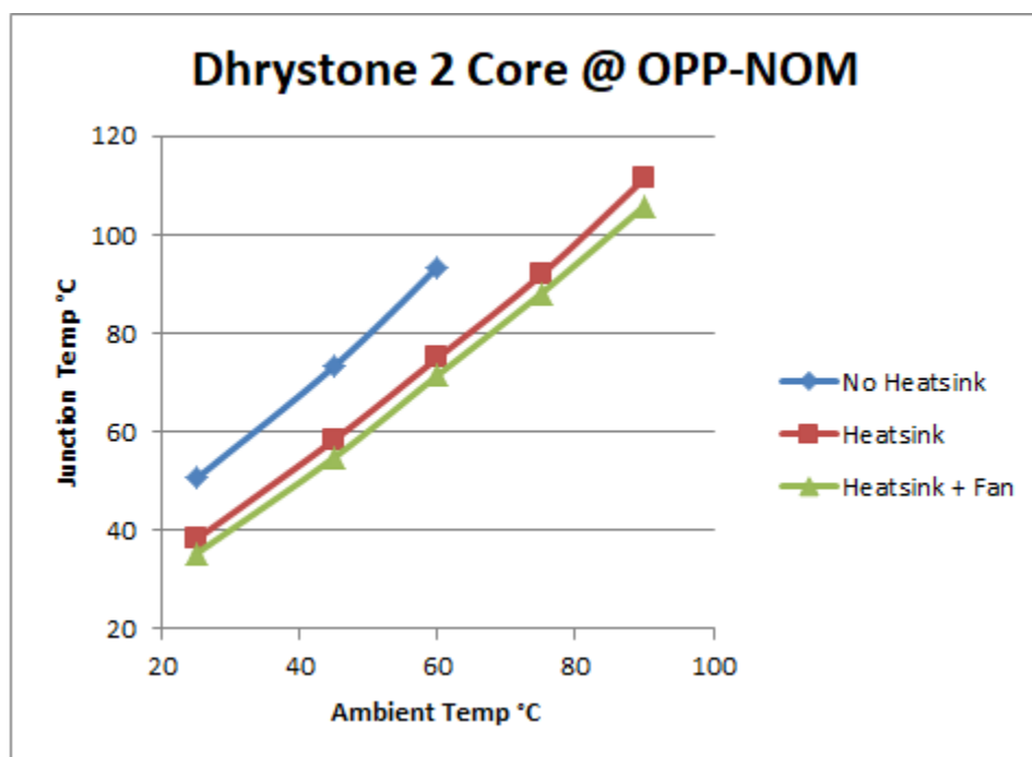
Figure 5. Dyrystone (Core 1 and Core 2) at OPP_NOM (Junction Temp vs Ambient Temp)
