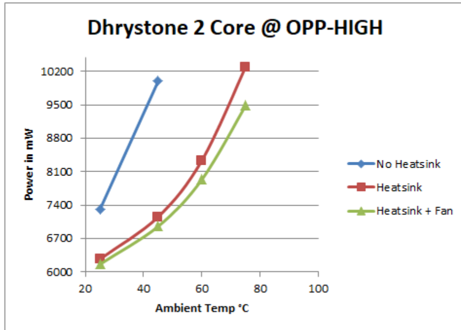
Figure 10. Dyrystone (Core 1 & Core 2) at OPP_HIGH (Power Consumption vs Ambient Temp)
