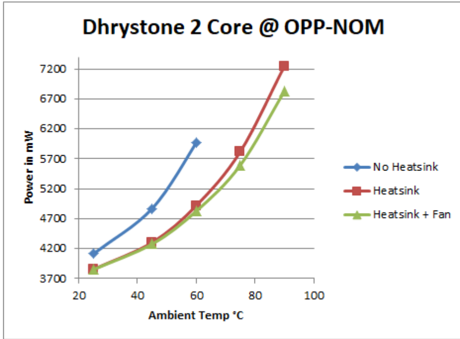
Figure 6. Dyrystone (Core 1 & Core 2) at OPP_NOM (Power Consumption vs Ambient Temp)
