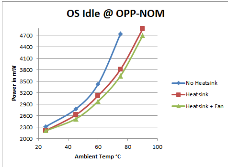
Figure 2. OS Idle - OPP_NOM (Power Consumption vs Ambient Temp)
