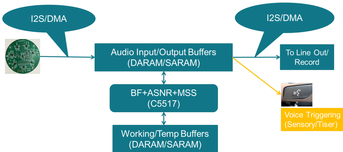
Figure 1. Demo Setup
