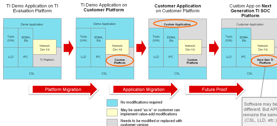
Figure 4. Maximize Software Reuse
