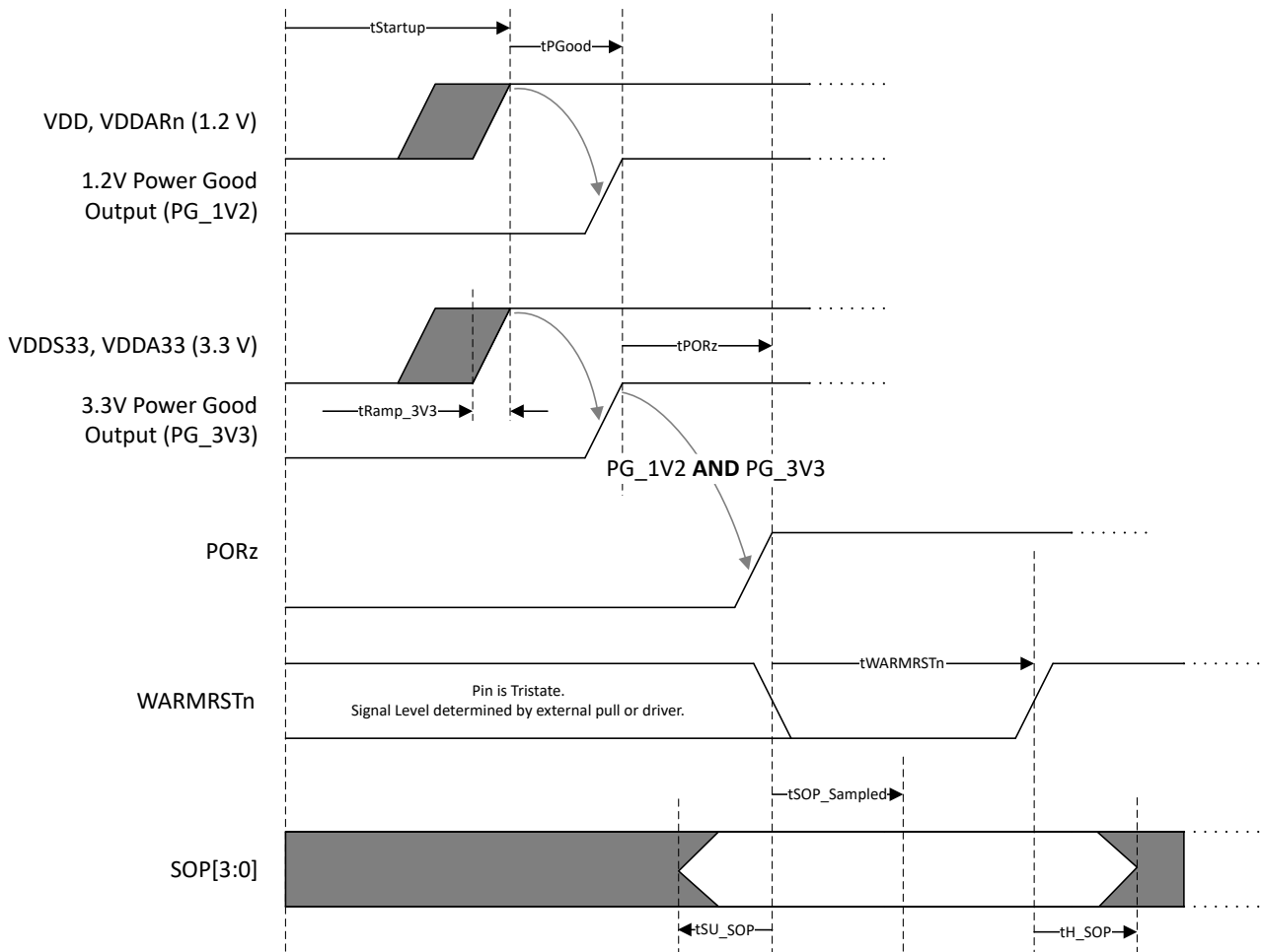
Figure 2-1. AM26x Power-On Sequencing
