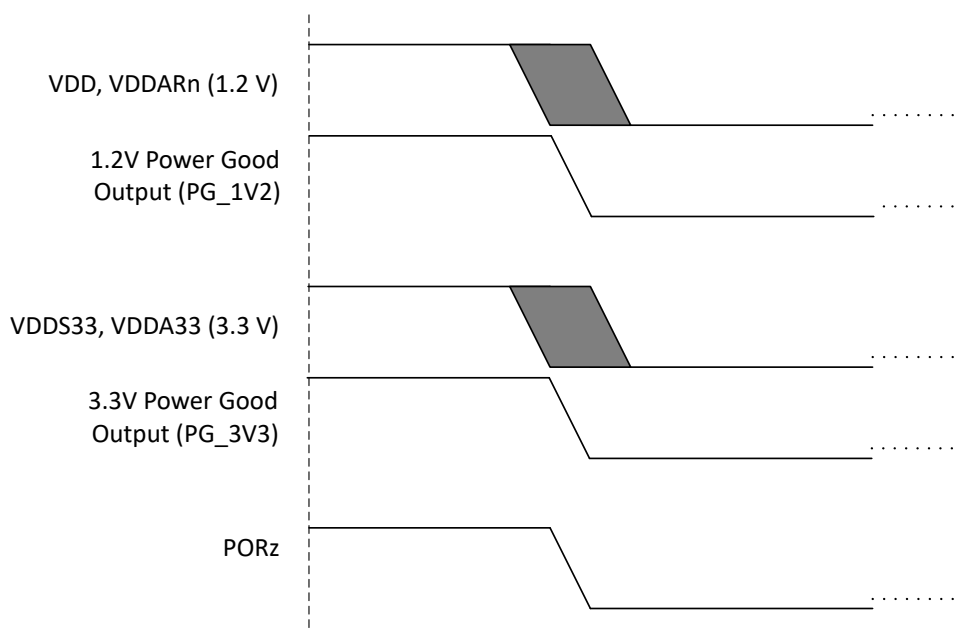
Figure 2-2. Power-Down Sequencing
