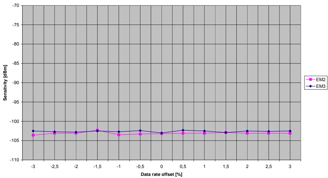
Figure 4. Sensitivity at PER 1% versus Data Rate Offset
