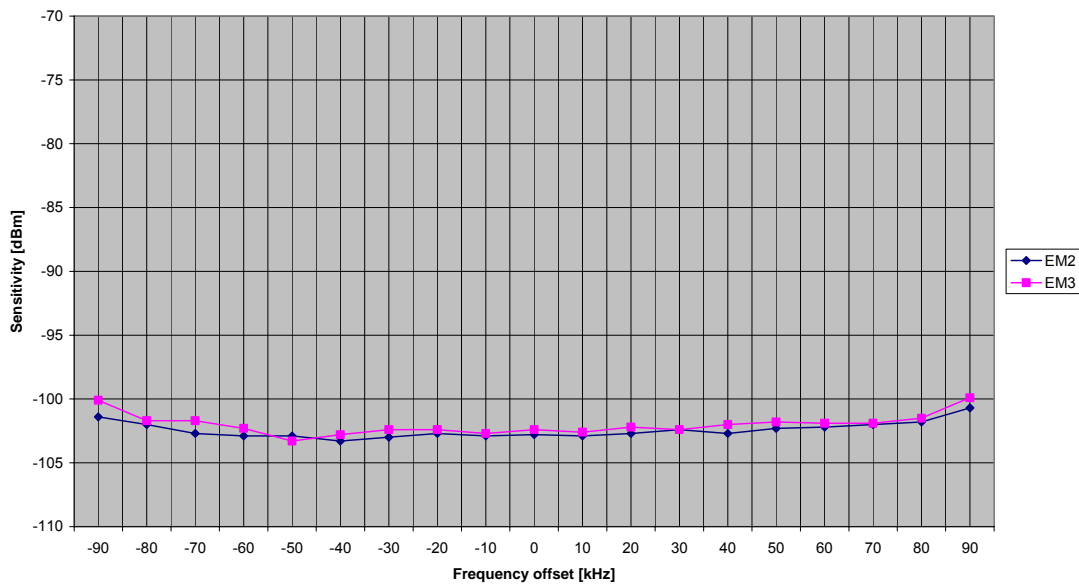
Figure 6. Sensitivity at PER 1 % versus Frequency Offset
