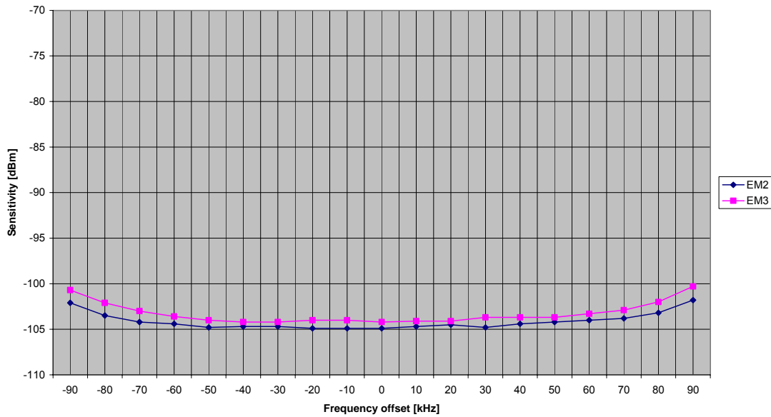
Figure 5. Sensitivity at PER 20 % versus Frequency Offset
