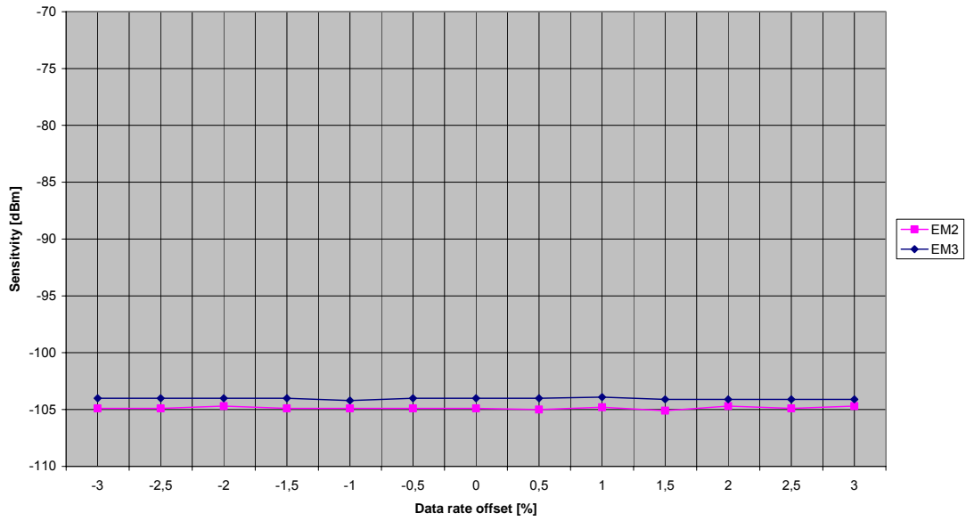
Figure 3. Sensitivity at PER 20 % versus Data Rate Offset
