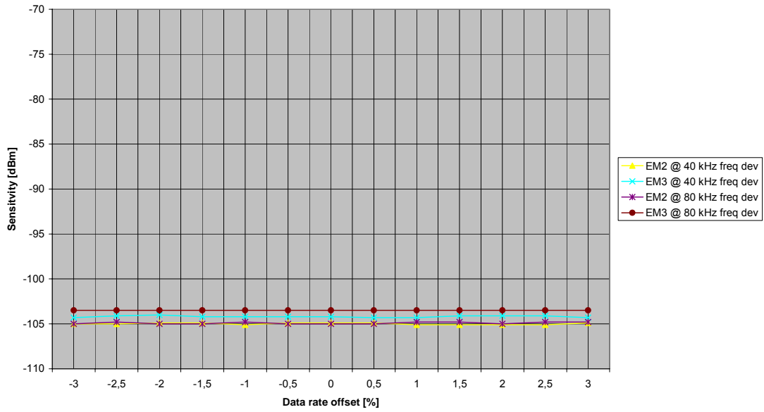
Sensitivity versus Data Rate Offset PER 20 %
