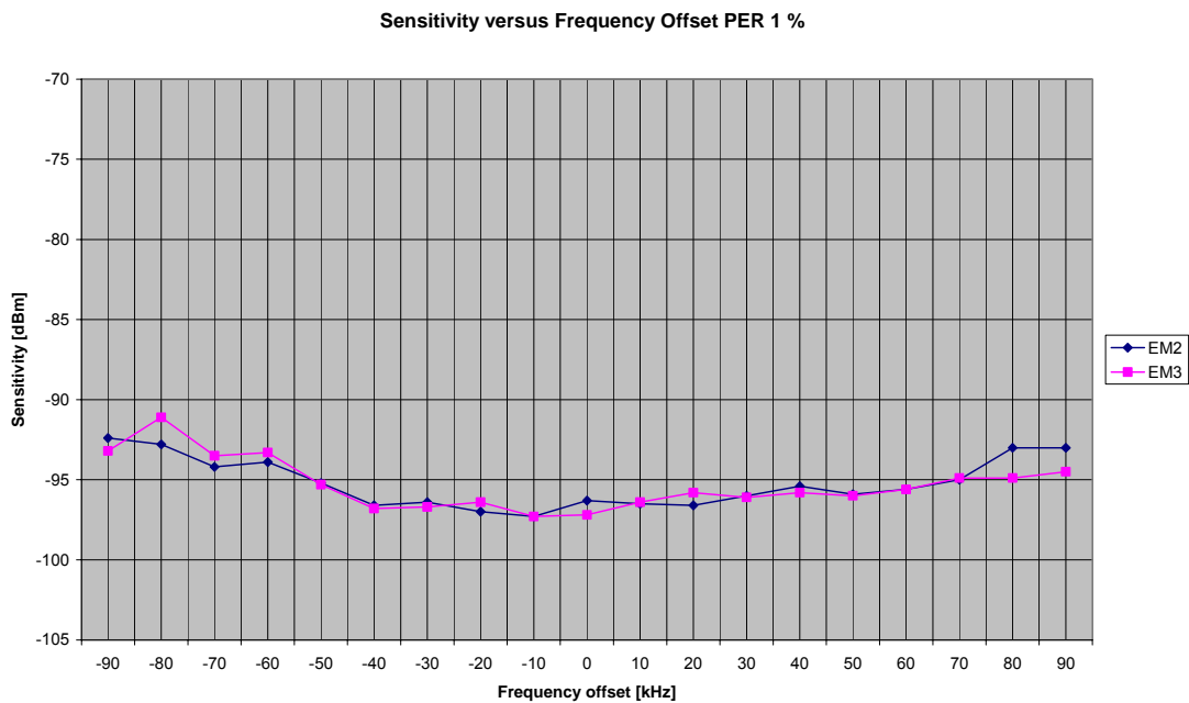
Figure 11. Sensitivity at PER 1% versus Frequency Offset
