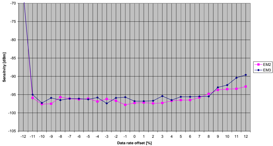
Figure 9. Sensitivity at PER 1% versus Data Rate Offset
