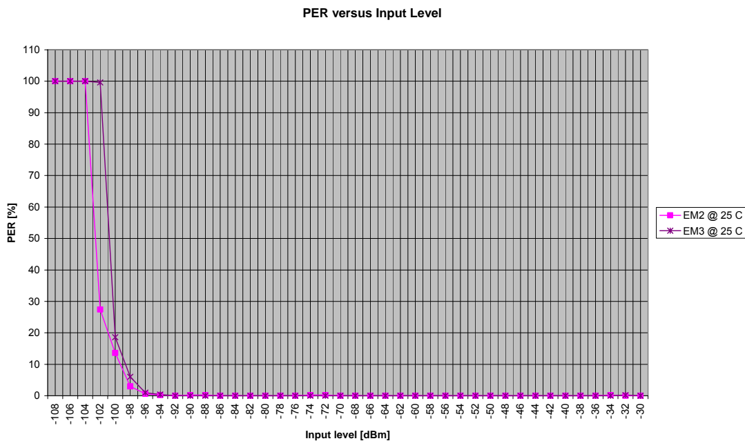
Figure 7. Sensitivity Curve
