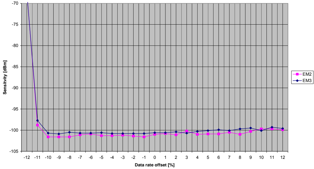
Figure 8. Sensitivity at PER 20% versus Data Rate Offset
