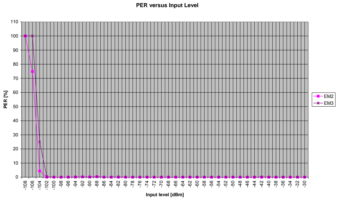
Figure 2. Sensitivity Curve
