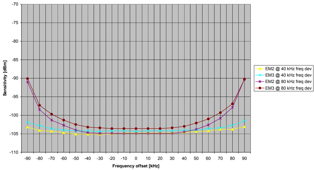
Sensitivity versus Frequency Offset PER 20 %
