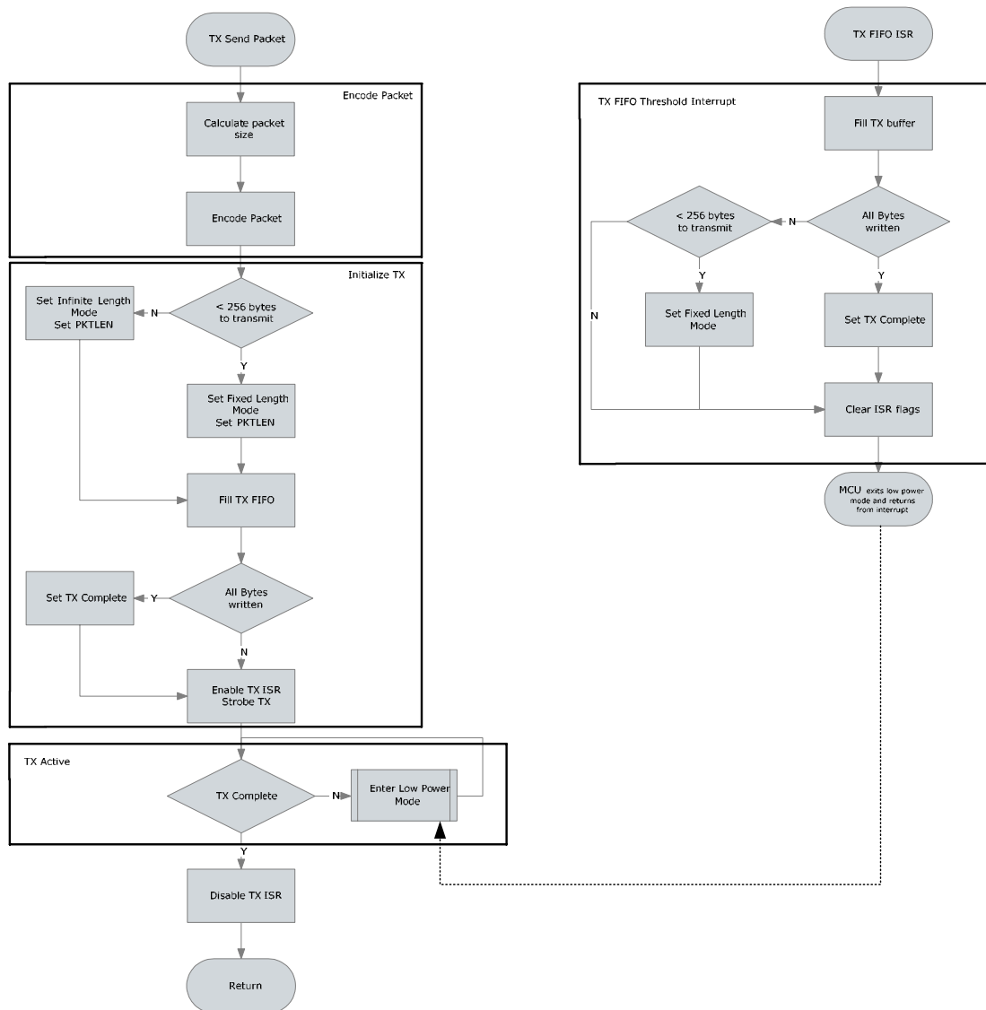
Figure 12. TX Flow Diagram
