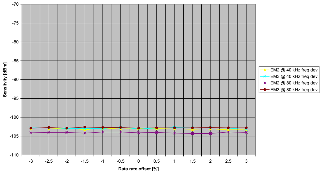
Sensitivity versus Data Rate Offset PER 1 %
