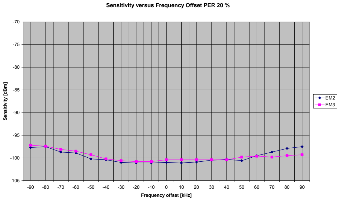
Figure 10. Sensitivity at PER 20% versus Frequency Offset
