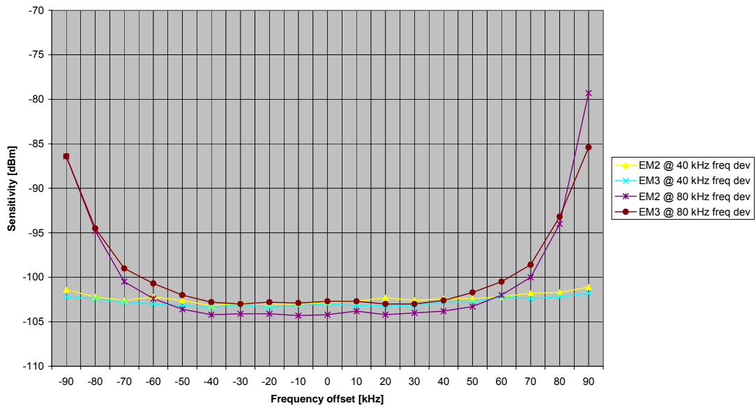
Sensitivity versus Frequency Offset PER 1 %
