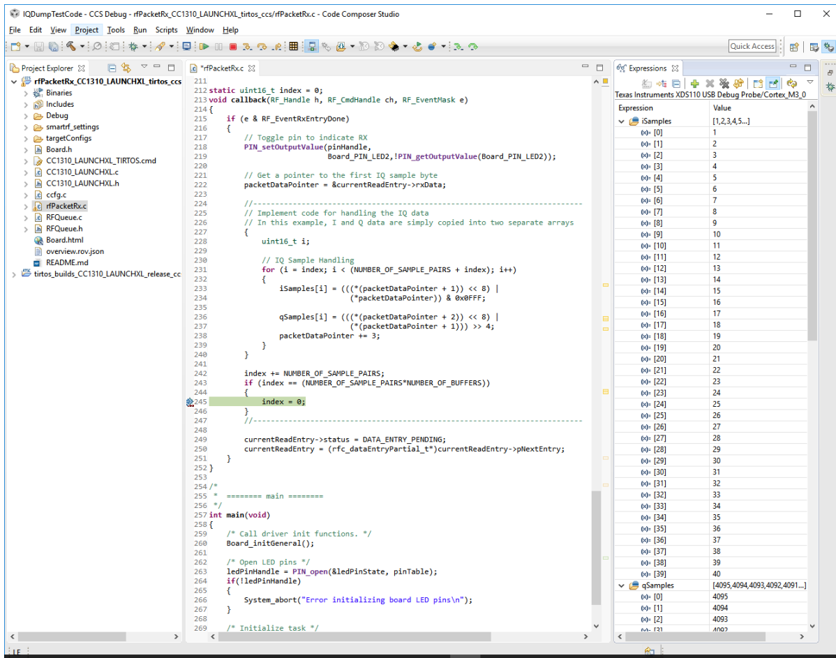
Figure 4-1. Built-In Test Pattern Stored as I and Q Samples
