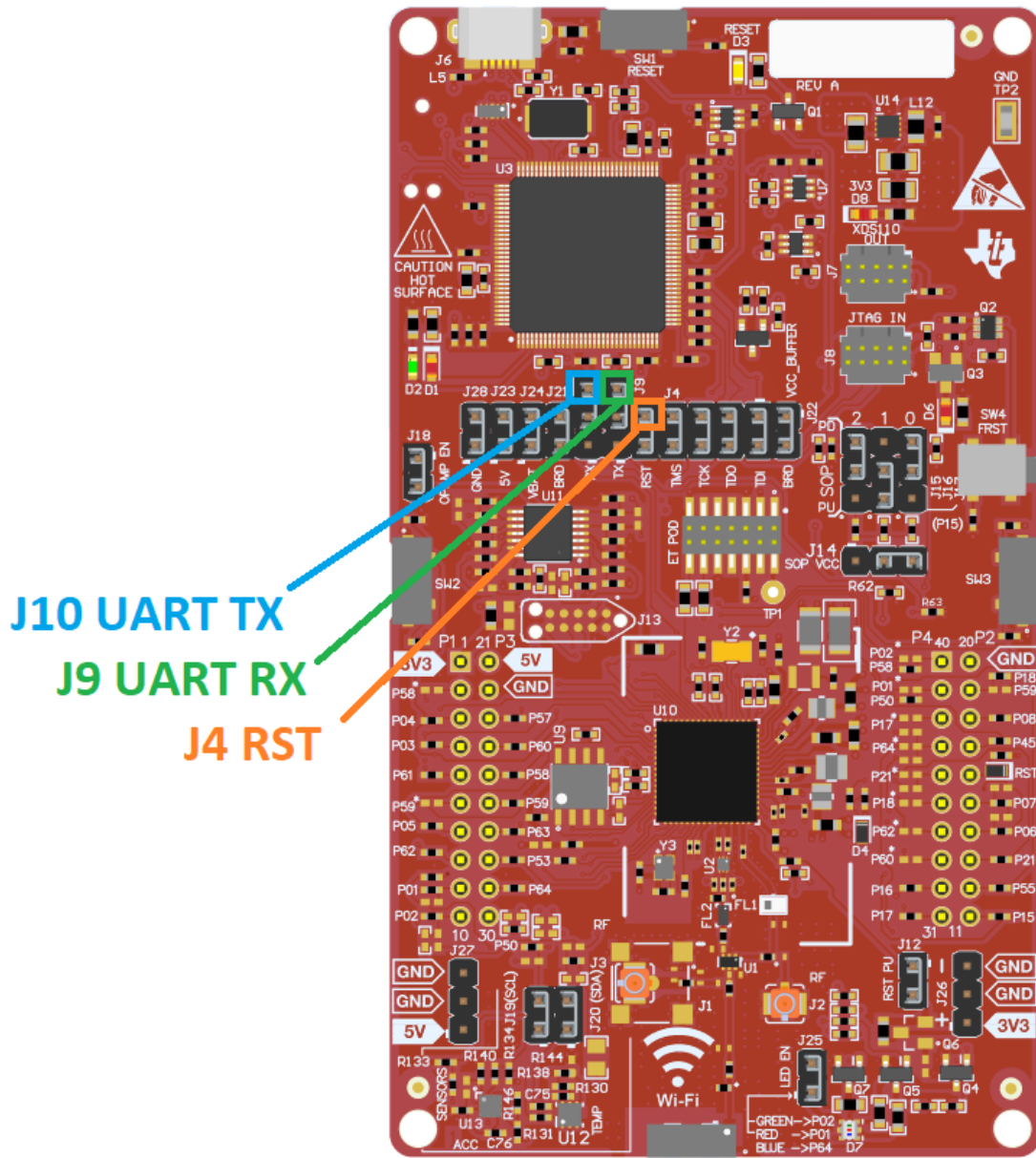
Figure 5-2. CC3235 LaunchPad™
