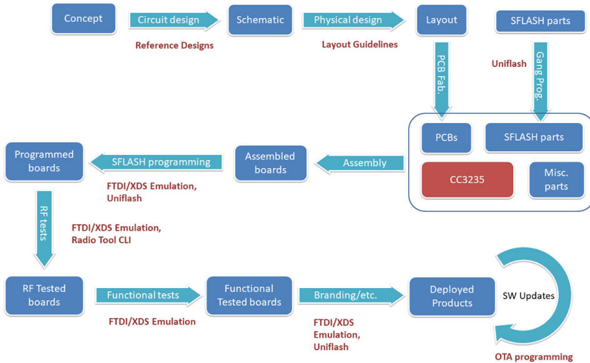
Figure 1-1. Production Line Overview
