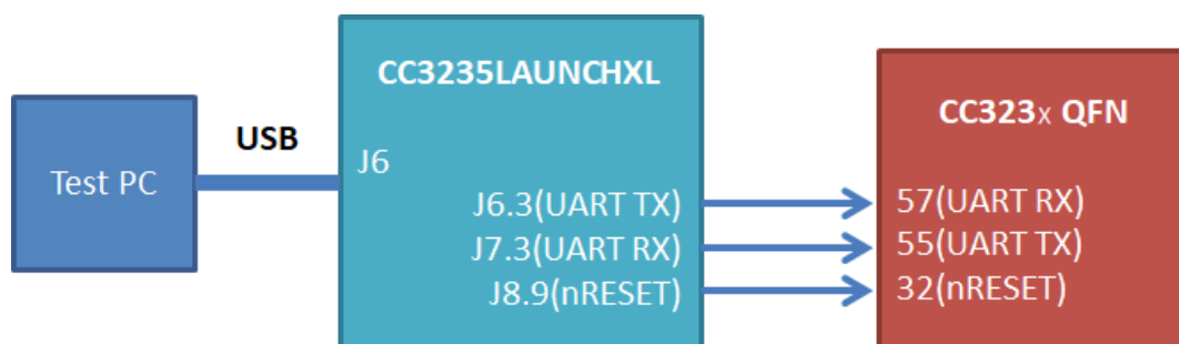
Figure 5-1. Connecting Through USB
