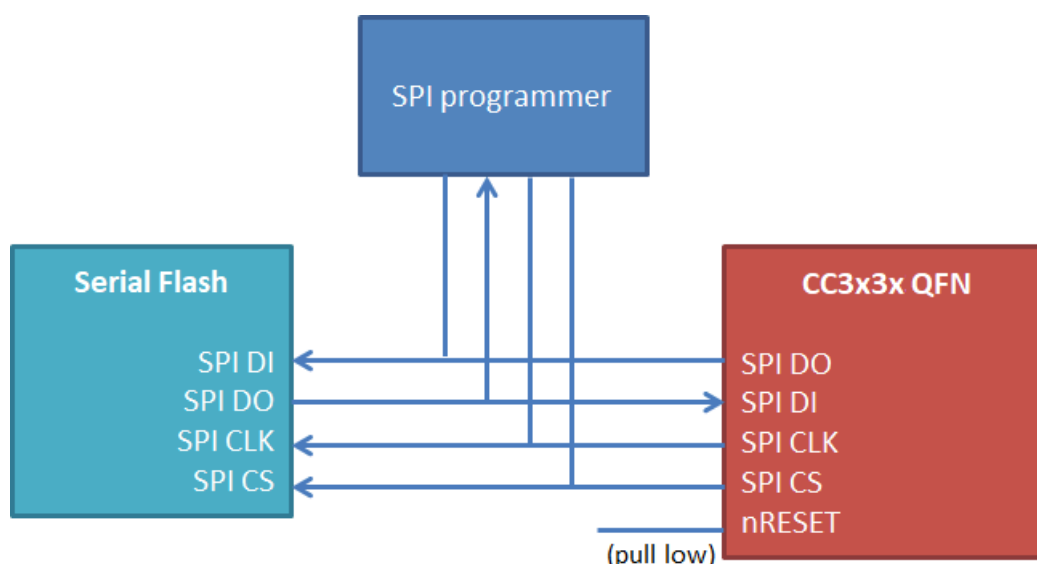
Figure 4-1. Programming Through SPI
