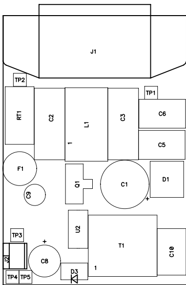
PMP2101 REV A
