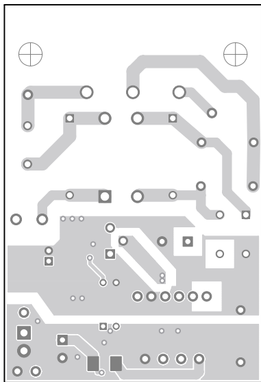
PMP2101 REV ALAYER 1-TOP
