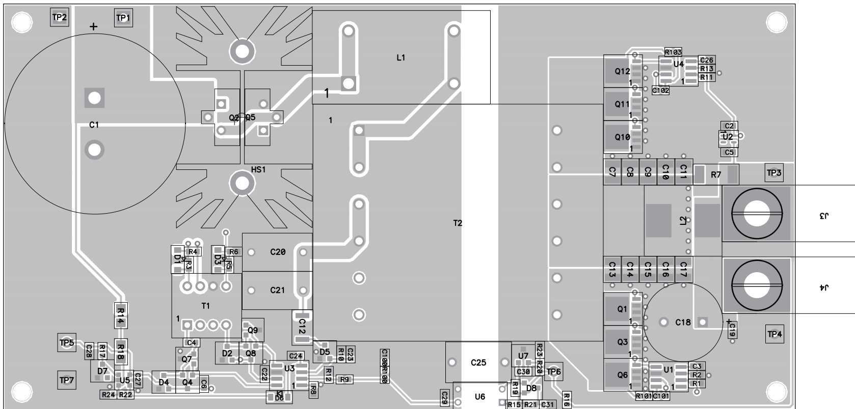
PMP5967 REV C TOP-LAYER 1
