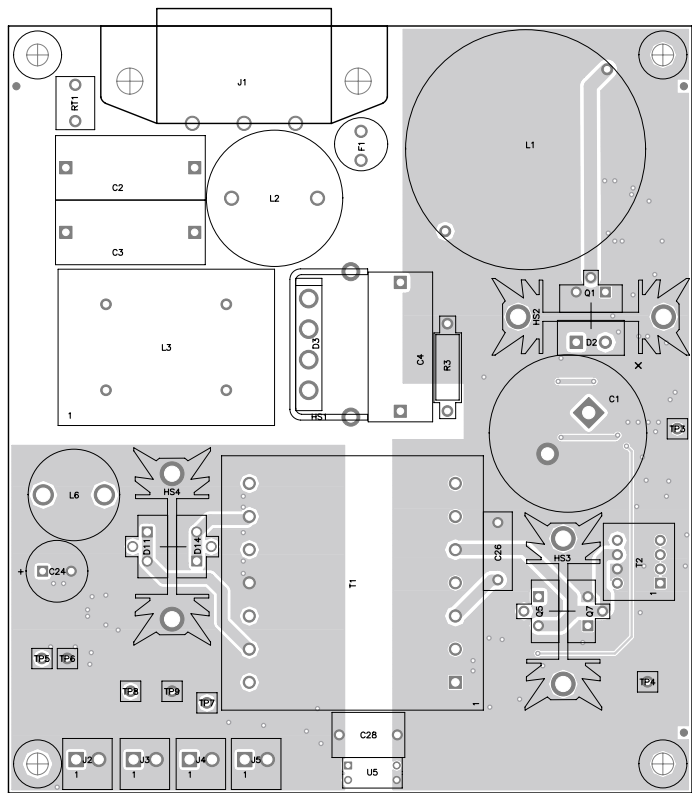
PMP5327 REV CLAYER 1-TOP
