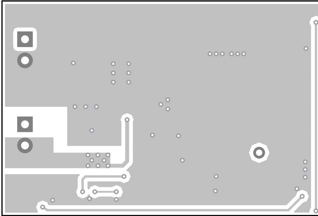
PMP4908 REV A
