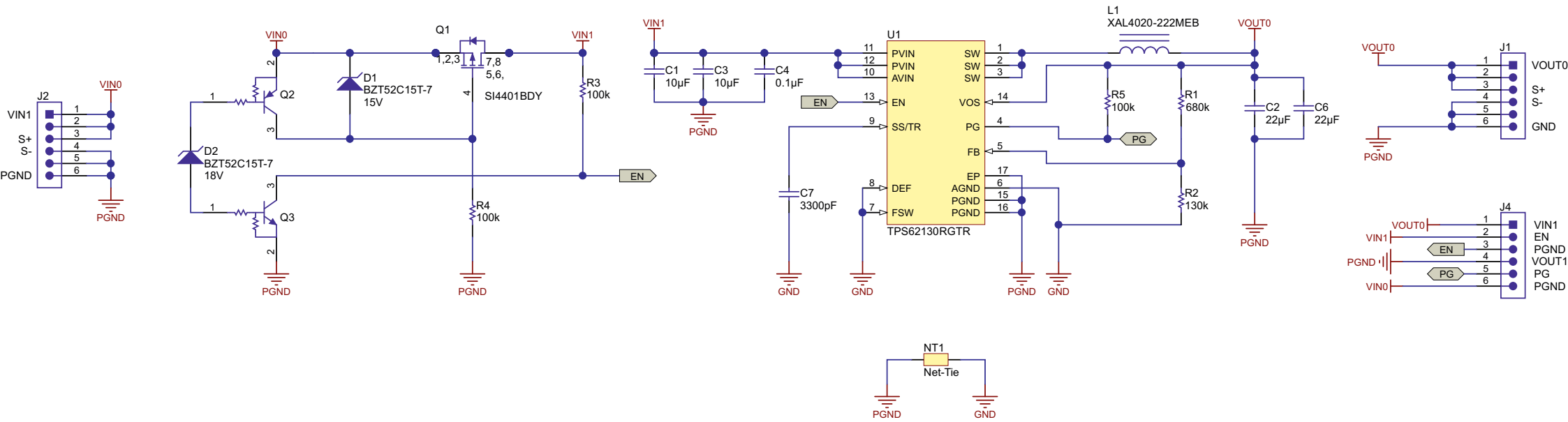
PMP9757 Step Down Converter with Input Overvoltage Protection
