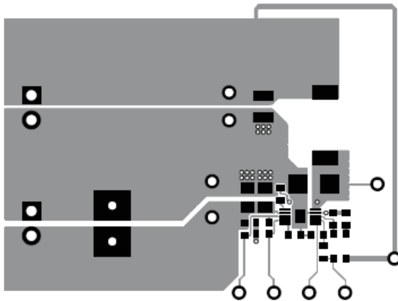
Figure 1. Top-Side Layout
