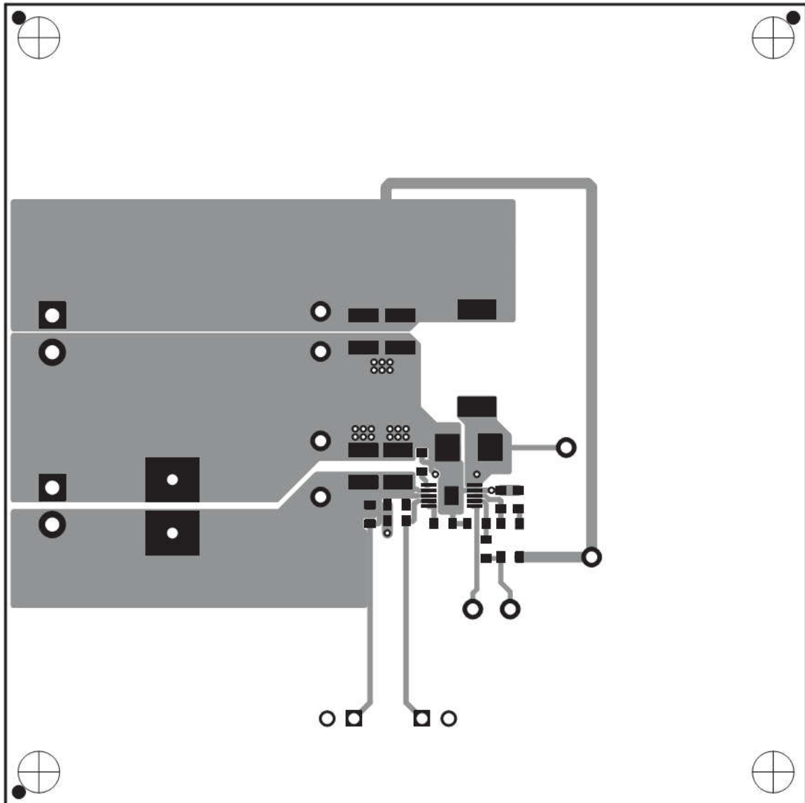
Figure 14. TPS54260EVM-597 Top-Side Layout
