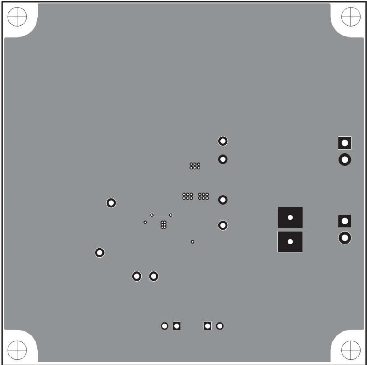
Figure 15. TPS54260EVM-597 Bottom-Side Layout
