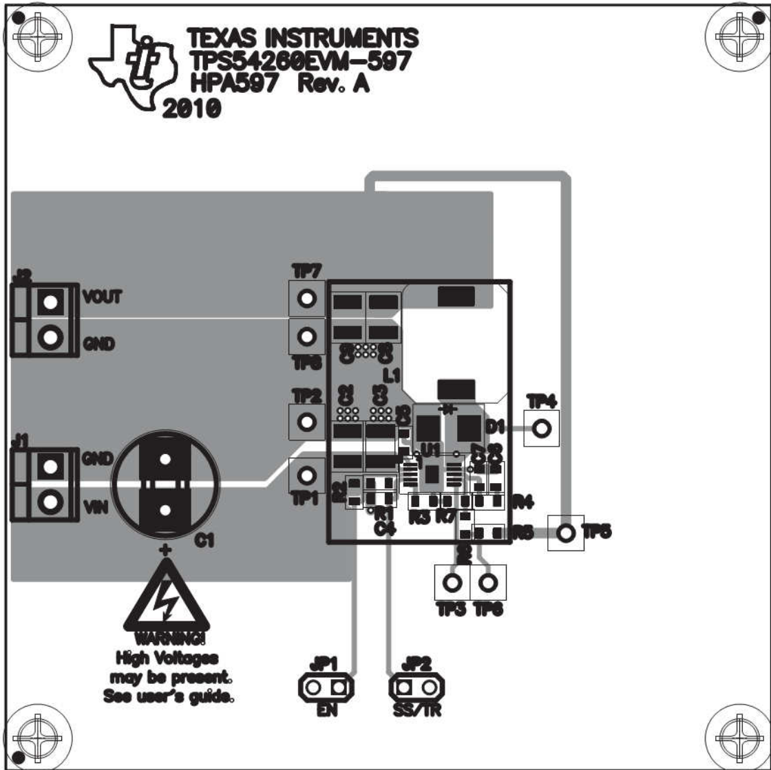
Figure 13. TPS54260EVM-597 Top-Side Assembly
