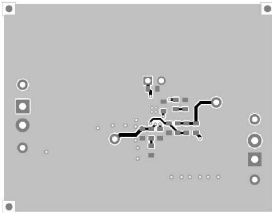
Figure 2: PMP8750_RevB_5 Bottom-Side Layout
