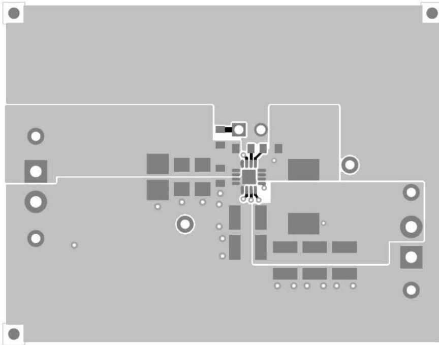
Figure 1: PMP8750_RevB_5 Top-Side Layout
