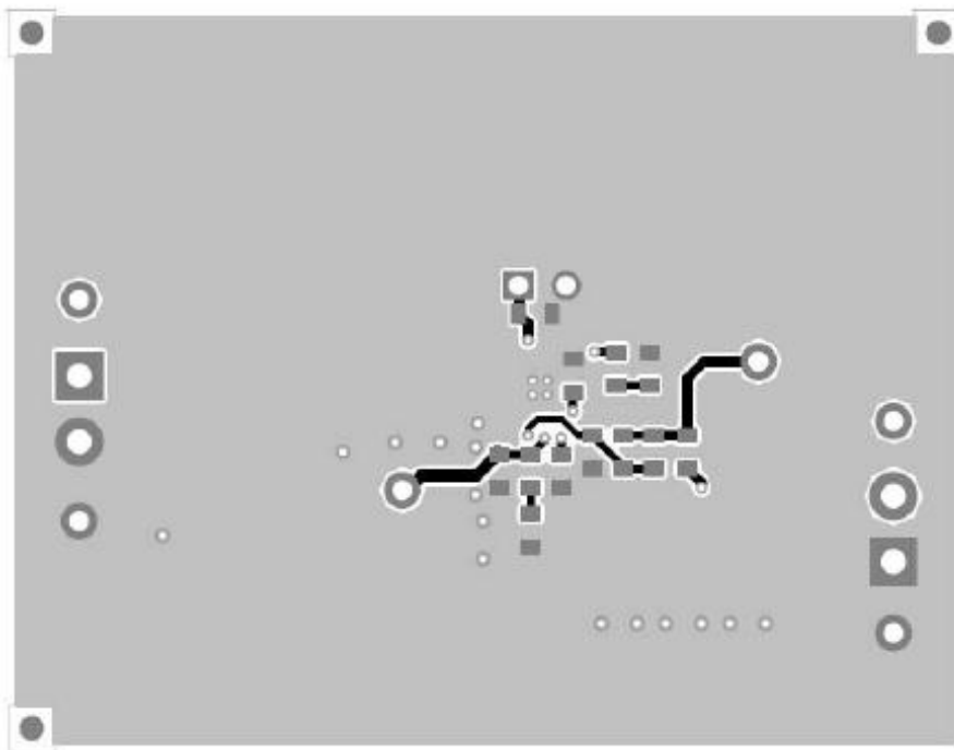
Figure 2: PMP8750_RevB_6 Bottom-Side Layout
