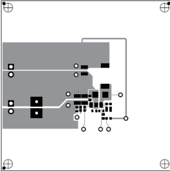
Figure 1: PMP8750_RevB_7 Top-Side Layout
