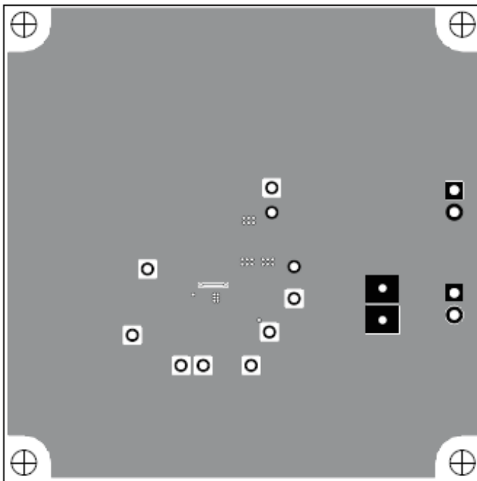
Figure 2: PMP8750_RevB_7 Bottom-Side Layout
