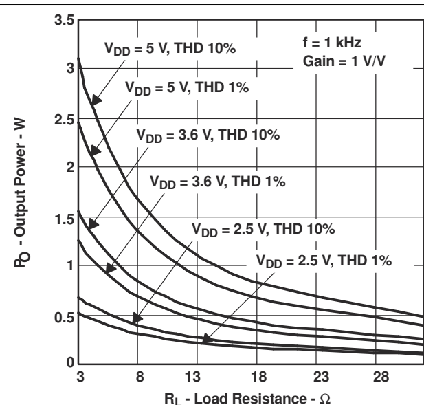
Figure 5-2. Output Power vs Load Resistance
