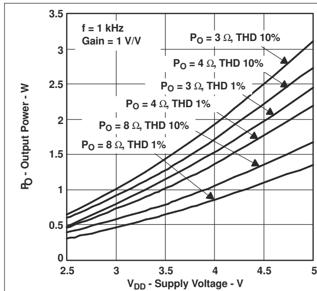
Figure 5-1. Output Power vs Supply Voltage
