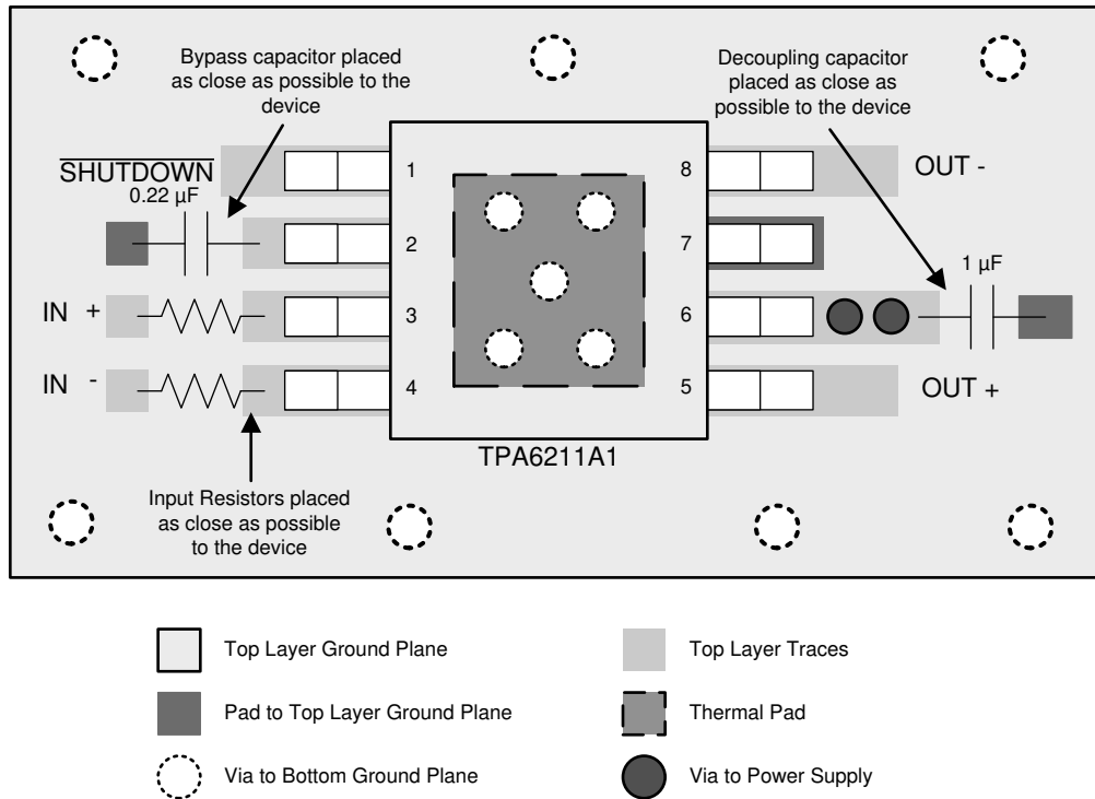
Figure 9-1. TPA6211A1-Q1 8-Pin HVSSOP (DGN) Board Layout
