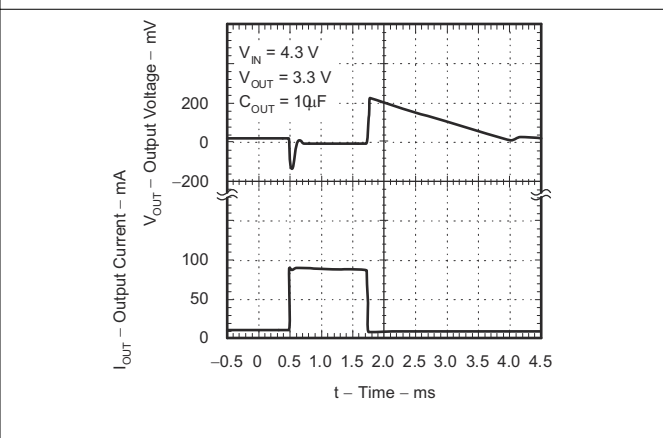
Figure 5-30. Load Transient Response (Legacy Chip)
