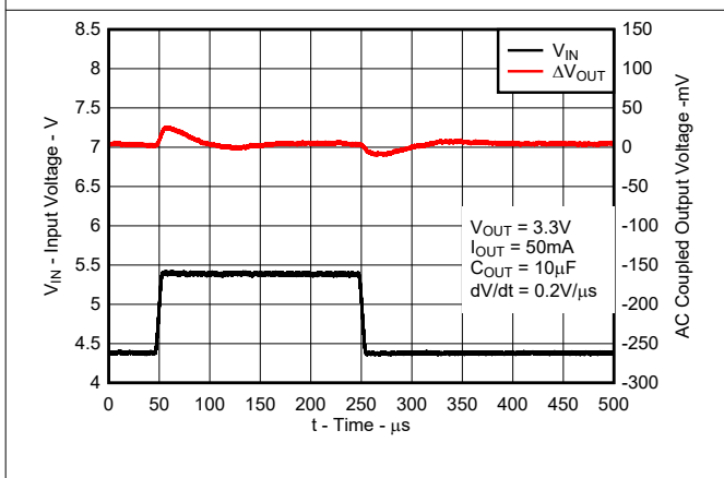
Figure 5-29. Line Transient Response (New Chip)
