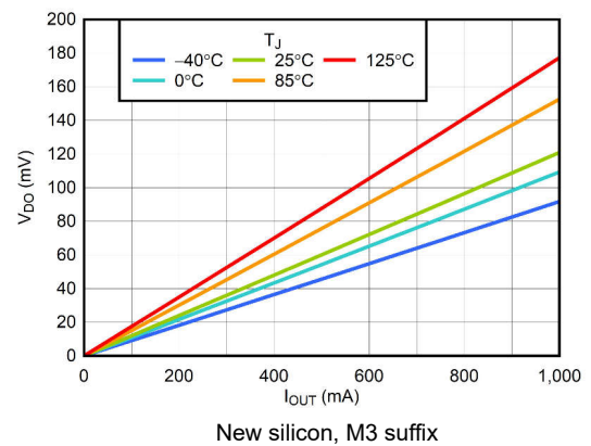
New silicon, M3 suffix Figure 5-6. Dropout Voltage vs Output Current
