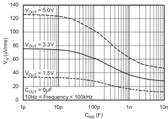
Figure 5-29. RMS Noise Voltage vs C_{NR}
