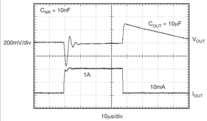
Figure 5-30. TPS73733 Load Transient Response
