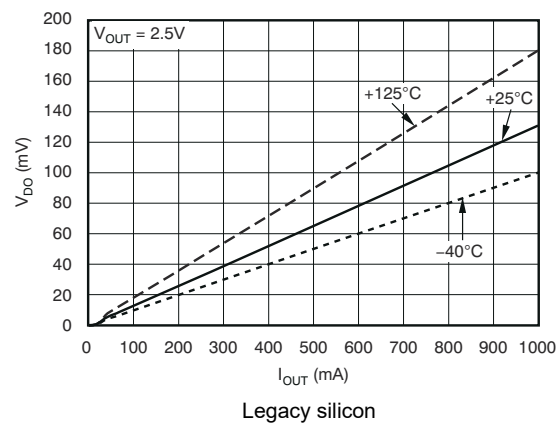
Legacy silicon Figure 5-5. Dropout Voltage vs Output Current
