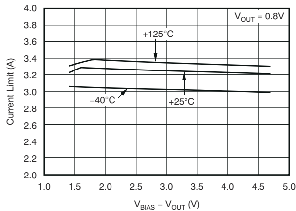
Figure 6-17. Current Limit vs (V_{BIAS} - V_{OUT})
