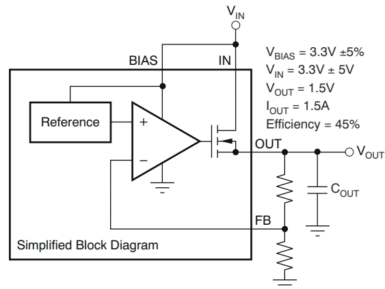
Figure 8-8. Typical Application of the TPS748 Without an Auxiliary Bias Rail
