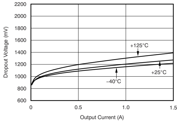
Figure 8-9. V_{BIAS} Dropout Voltage vs I_{OUT} and Temperature ( T_J )
