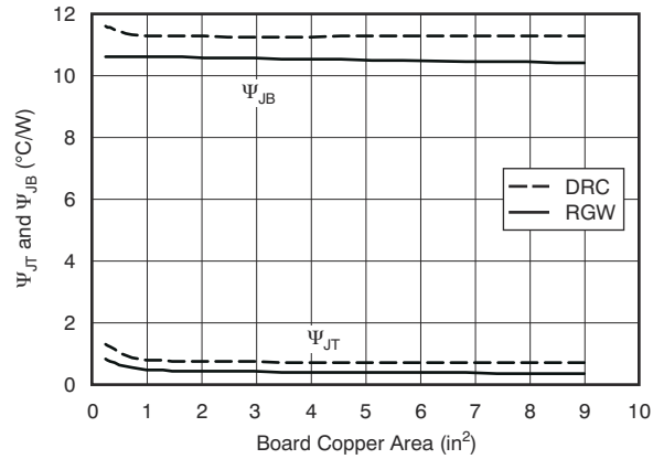
Figure 8-15. \Psi_{JT} and \Psi_{JB} vs Board Size
