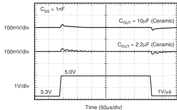
Figure 8-12. V_{BIAS} Line Transient
