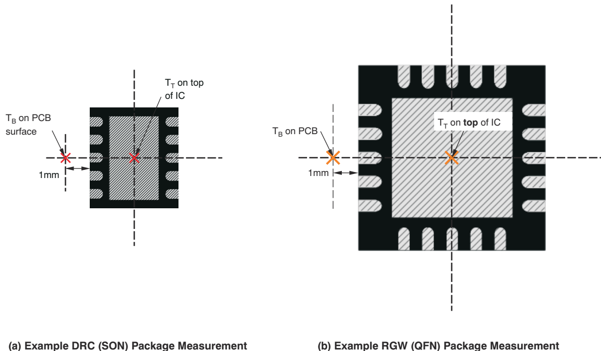
Figure 8-14. Measuring Points for T_T and T_B
