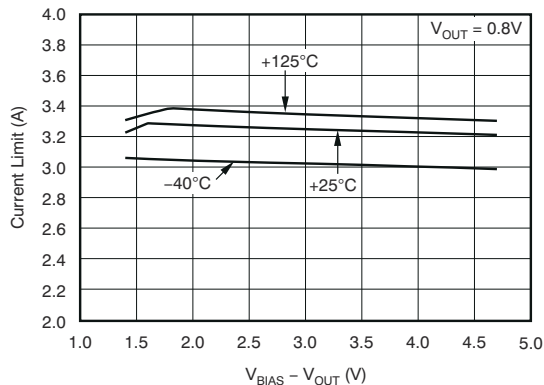
Figure 8-11. Current Limit vs ( V_{BIAS} - V_{OUT} )
