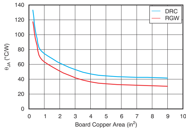
Figure 8-13. R_{\theta JA} vs Board Size
