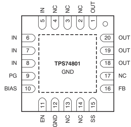
Figure 5-2. RGW Package, 20-Pin VQFN (Top View)
