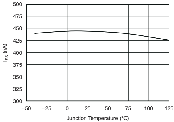
Figure 6-15. Soft-Start Charging Current ( I_{SS} ) vs Temperature ( T_J )
