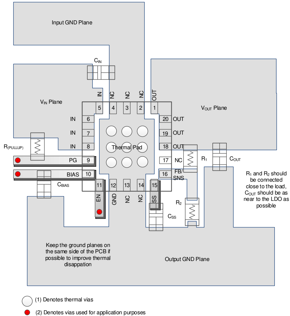
Figure 8-16. Layout Example (RGW Package)
