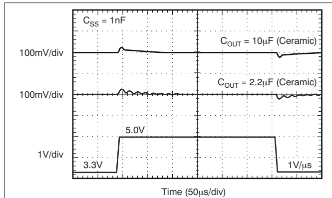
Figure 8-3. V_{BIAS} Line Transient
