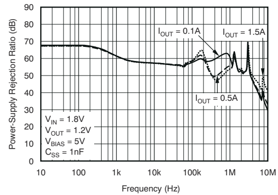
Figure 8-10. V_{BIAS} PSRR vs Frequency
