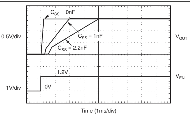
Figure 8-6. Turn-On Response
