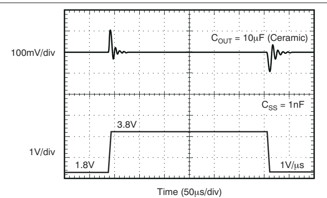
Figure 8-4. V_{IN} Line Transient
