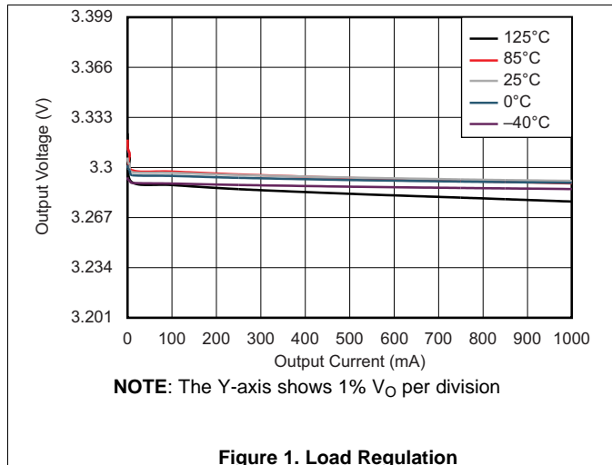
Figure 1. Load Regulation
