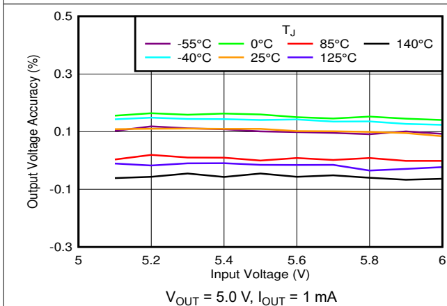
Figure 6-29. Output Accuracy vs V_{IN} and Temperature
