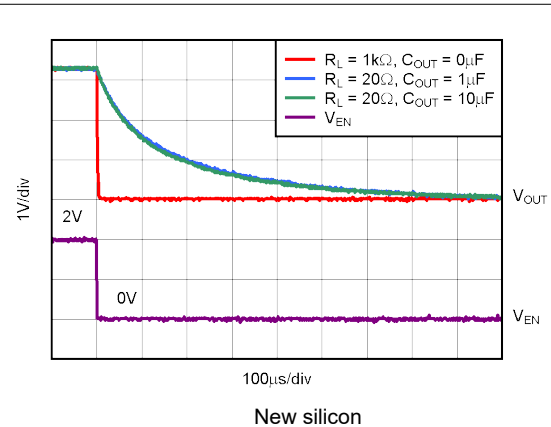
Figure 5-42. TPS73233-Q1 Turn-Off Response
