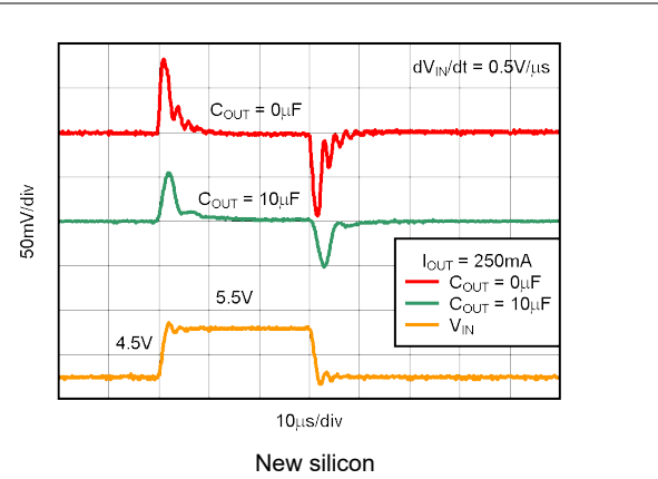
Figure 5-38. TPS73233-Q1 Line Transient Response
