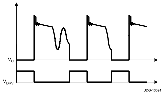
Figure 18. Valley-Skipping Mode
