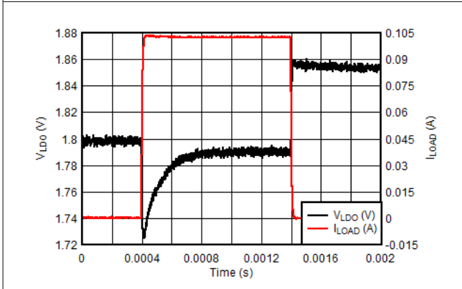
Figure 10-18. LDO Load Transient - VLDO = 1.8V
