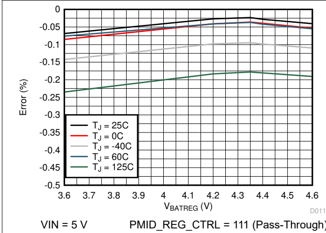
Figure 8-1. Battery Regulation Voltage Accuracy vs. VBATREG Setting
