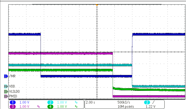
Figure 10-5. Power Up from Ship Mode with MR Bar Press
