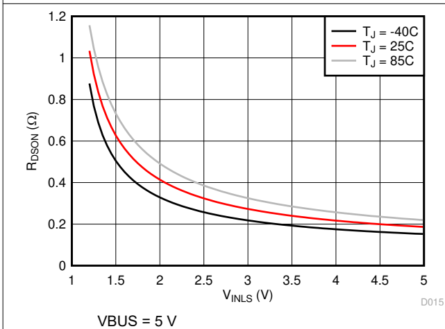
Figure 8-5. LS/LDO Switch On Resistance vs. VINLS
