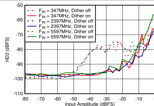
Figure 5-78. Dual Channel Mode: HD3 vs Input Amplitude and Dither
