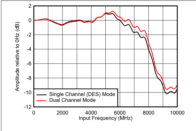
Figure 5-1. Input Amplitude vs Input Frequency
