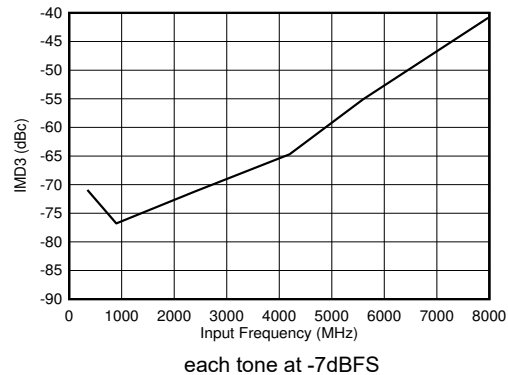
Figure 5-104. Dual Channel Mode: IMD3 vs Input Frequency
