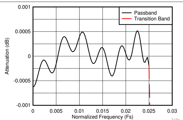
Figure 6-16. Decimate-by-16 Composite Zoomed Pass-Band Response
