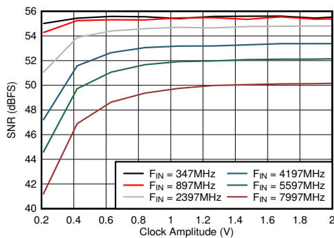
Figure 5-83. Dual Channel Mode: SNR vs Clock Amplitude
