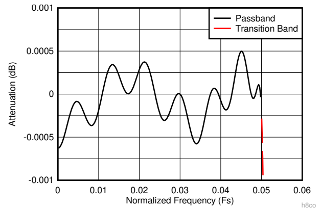
Figure 6-14. Decimate-by-8 Composite Zoomed Pass-Band Response
