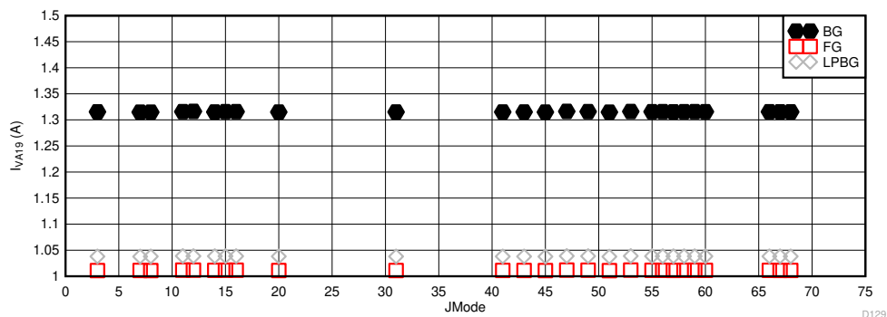
Figure 5-112. DES Mode: Power Dissipation vs JMODE at 10.4GSPS
