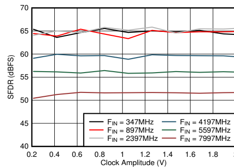
Figure 5-84. Dual Channel Mode: SFDR vs Clock Amplitude
