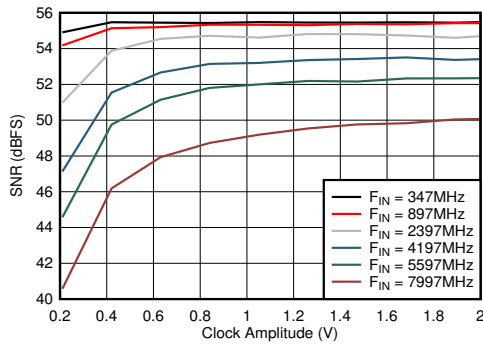
Figure 5-81. DES Mode: SNR vs Clock Amplitude
