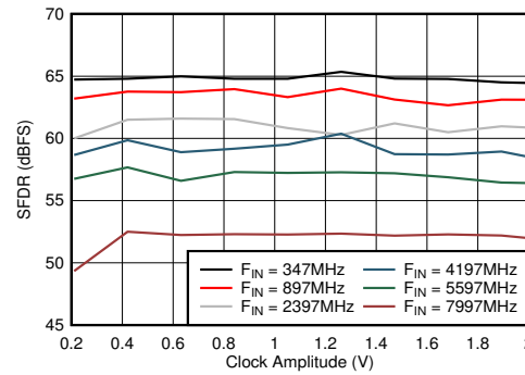
Figure 5-82. DES Mode: SFDR vs Clock Amplitude
