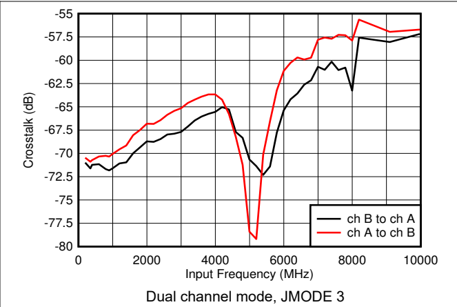
Figure 5-2. Crosstalk vs Input Frequency
