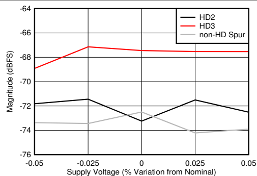
Figure 6-94. DES Mode: HD2, HD3 and Worst non-HD Spur vs Supply Voltage
