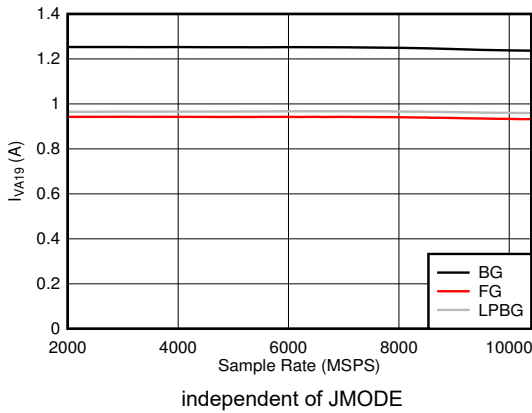
Figure 6-121. DES Mode: I_{VA19} vs Sample Rate
