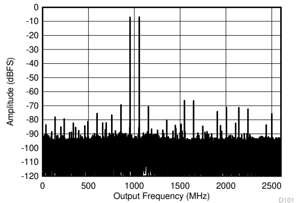
each tone at -7 dBFS, 100 MHz Tone Spacing
