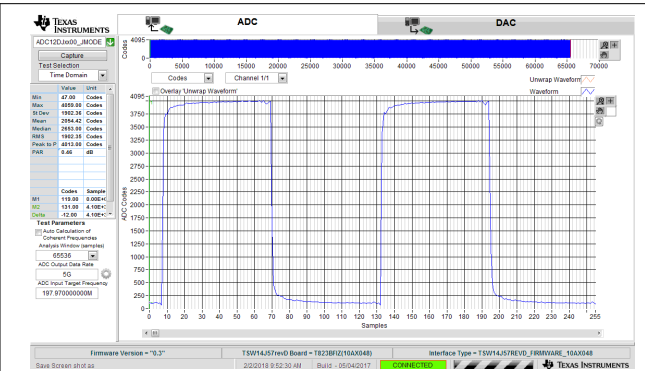
Figure 8-7. 40-MHz, Square-Wave Time Domain for 5-GSPS, Single-Channel Oscilloscope
