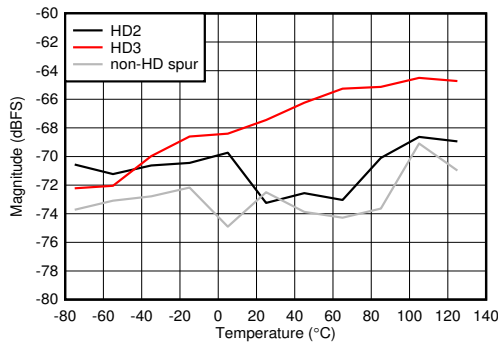
Figure 6-91. Dual Channel Mode: HD2, HD3 and Worst non-HD Spur vs Temperature
