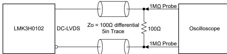
Figure 6-3. DC-LVDS Output Configuration During Device Test
