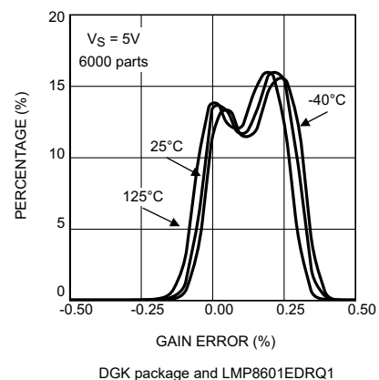
Figure 5-48. Gain Error Distribution at V_S = 5V LMP8601-Q1
