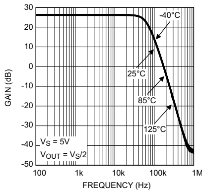
Figure 5-11. Gain vs Frequency at V_S = 5V
