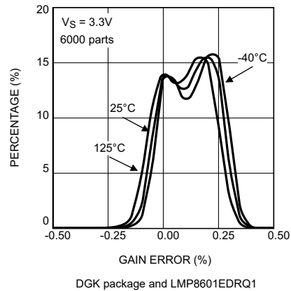
Figure 5-46. Gain Error Distribution at V_S = 3.3V LMP8601-Q1
