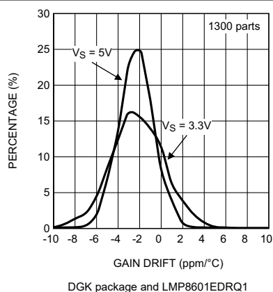
Figure 5-42. Gain Drift Distribution, 1300 Parts LMP8601-Q1
