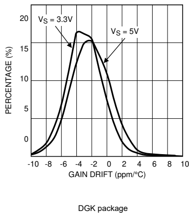
Figure 5-45. Gain Drift Distribution, 5000 Parts LMP8603-Q1
