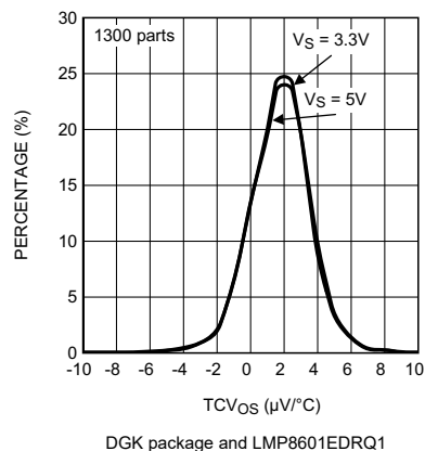
Figure 5-40. TCV_{OS} Distribution
