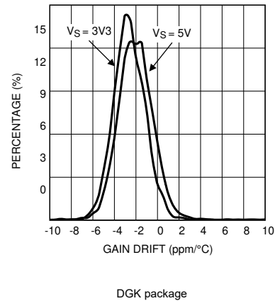
Figure 5-44. Gain Drift Distribution, 5000 Parts LMP8602-Q1
