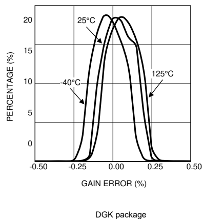
Figure 5-50. Gain Error Distribution at V_S = 3.3V , 5000 Parts LMP8602-Q1
