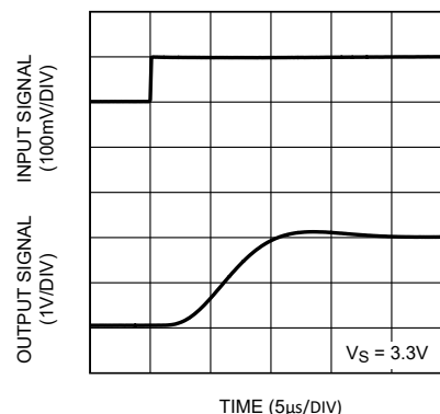
Figure 5-18. Settling Time (Rising Edge) at V_S = 3.3V LMP8601-Q1
