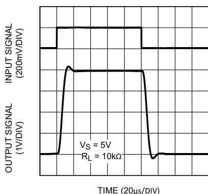
Figure 5-15. Step Response at V_S = 5V LMP8601-Q1
