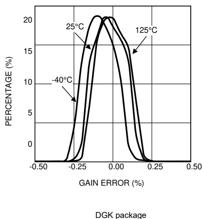
Figure 5-52. Gain Error Distribution at V_S = 5V , 5000 Parts LMP8602-Q1
