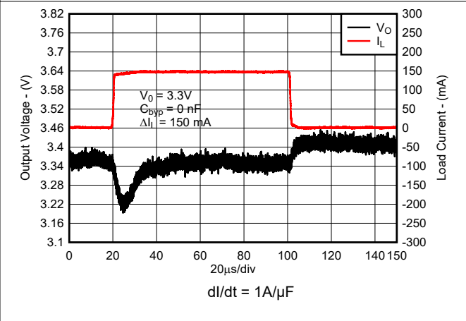
Figure 7-13. Load Transient Response (New Chip)
