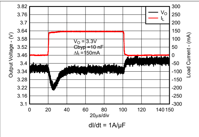
Figure 7-11. Load Transient (New Chip)
