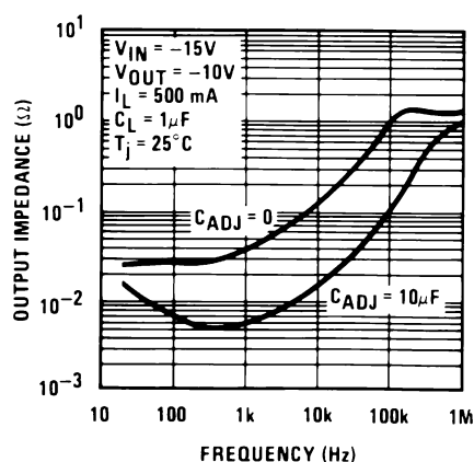
Figure 5-10. Output Impedance
