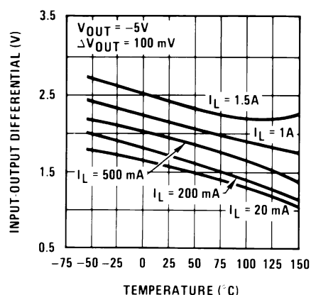
Figure 5-4. Dropout Voltage
