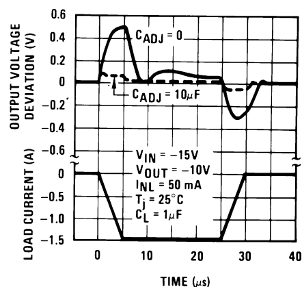
Figure 5-12. Load Transient Response
