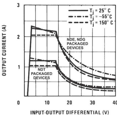
Figure 7-2. Current Limit
