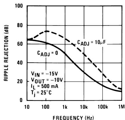
Figure 5-8. Ripple Rejection
