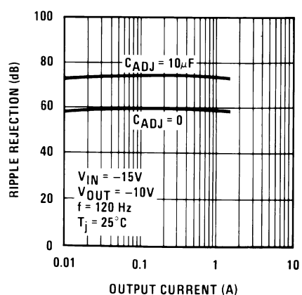
Figure 5-9. Ripple Rejection
