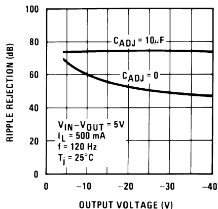
Figure 5-7. Ripple Rejection
