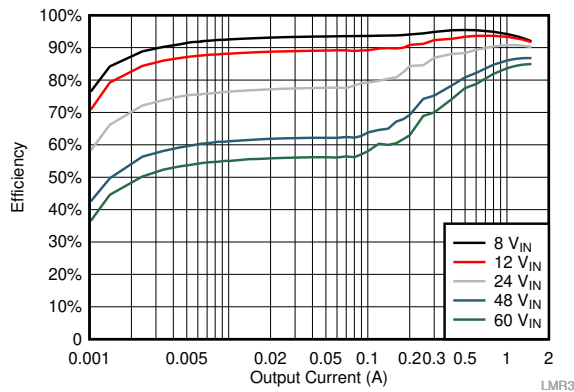
Figure 10-4. Efficiency
