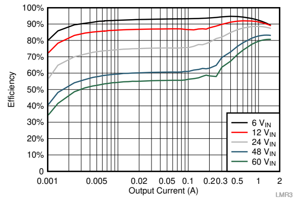
Figure 10-5. Efficiency
