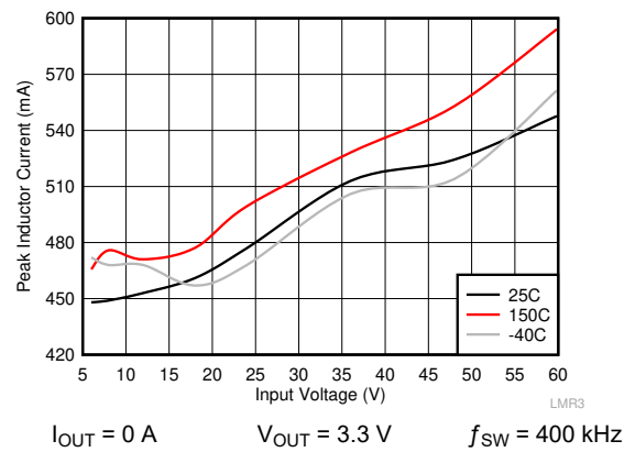
Figure 8-6. I_{PEAK-MIN}
