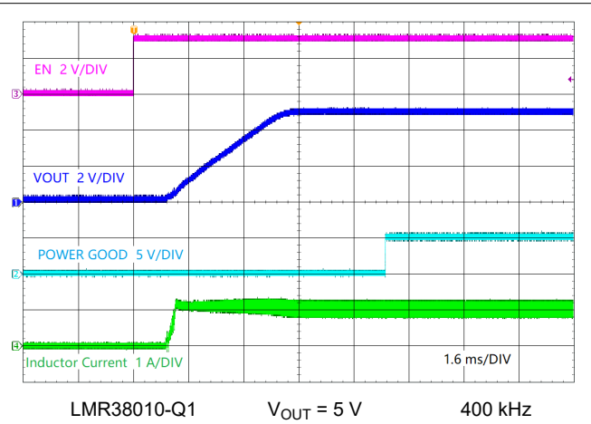
Figure 8-4. Start-Up by EN
