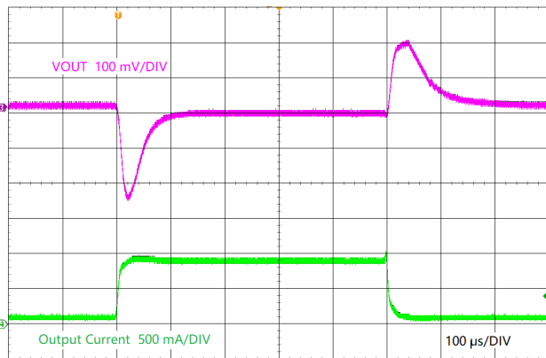
LMR38010-Q1 V_{OUT} = 5\text{ V} 400 kHz (AC Coupled) 100 mA to 900 mA at 200 mA/μs
