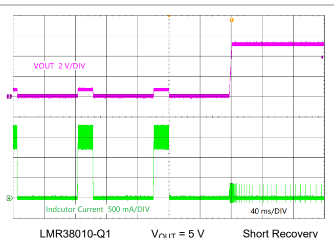
Figure 8-8. Short-Circuit Recovery
