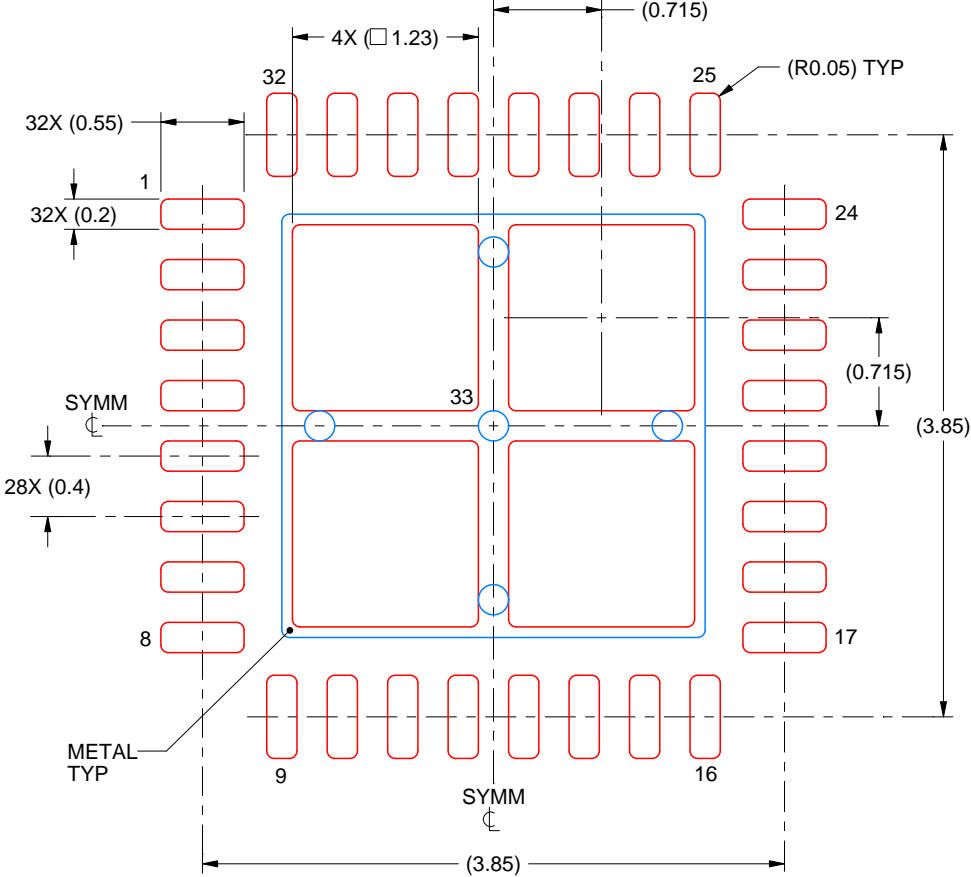
SOLDER PASTE EXAMPLE BASED ON 0.1 mm THICK STENCIL EXPOSED PAD 33: 77% PRINTED SOLDER COVERAGE BY AREA UNDER PACKAGE SCALE:20X
