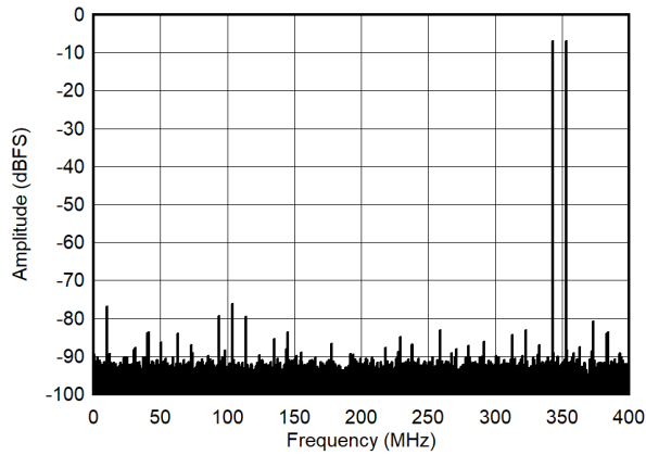
Figure 7-51. Single Tone FFT at 348 MHz
