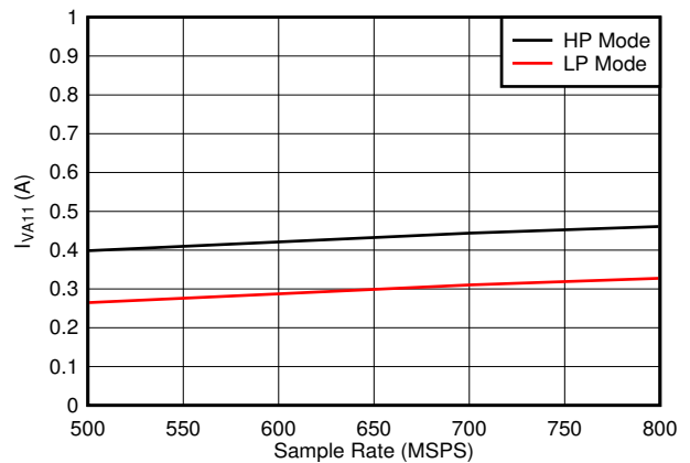
Figure 7-76. Quad Channel, I_{VA11} vs F_S Independent of JMODE
