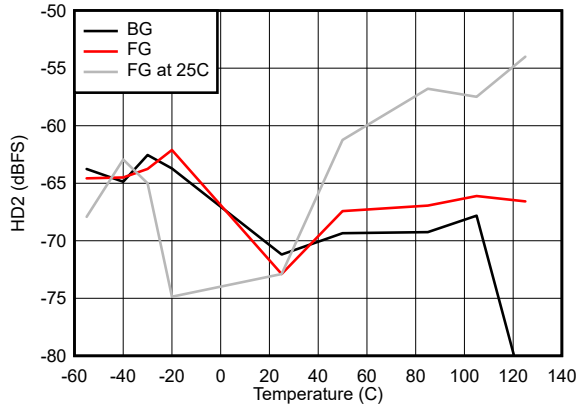
Low Power Mode, F_{IN} = 347 MHz
