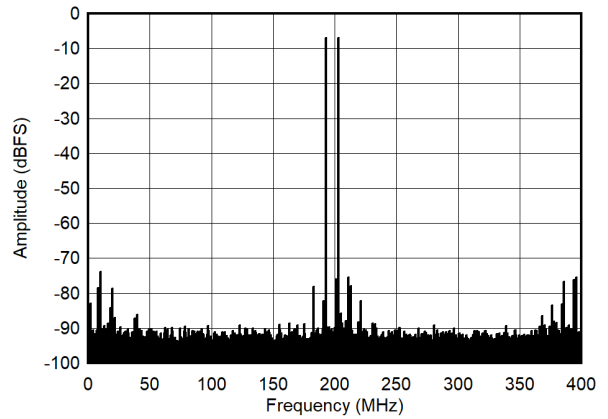
Figure 7-52. Single Tone FFT at 998 MHz
