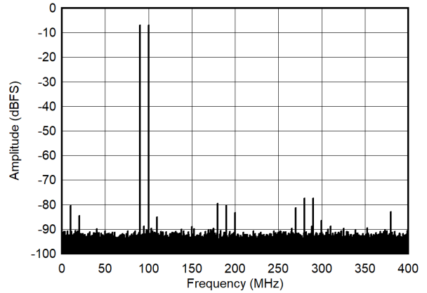
Figure 7-50. Single Tone FFT at 95 MHz
