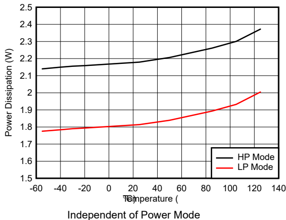
Figure 7-113. Quad Channel, Power Dissipation vs Temperature
