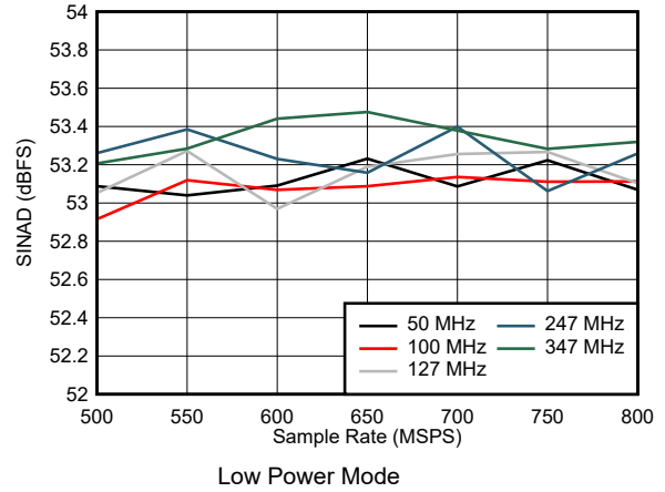
Figure 7-26. SINAD vs Sample Rate
