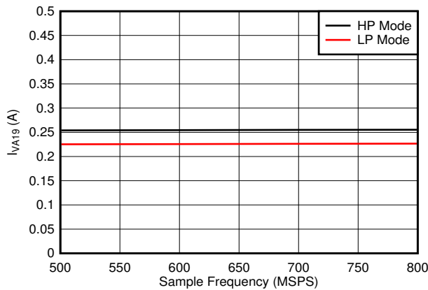
Figure 7-95. Single Channel, I_{VA19} vs F_S Independent of JMODE
