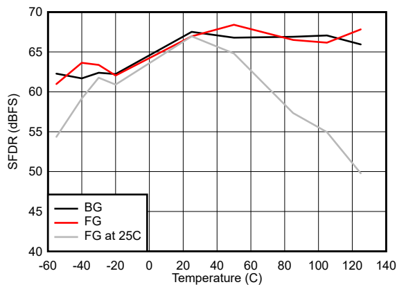
Figure 7-35. SFDR vs Temperature
