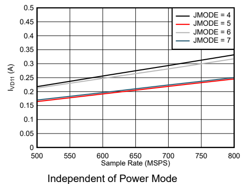
Figure 7-78. Quad Channel, I_{VD11} vs F_S for JMODES 4 - 7 Independent of Power Mode
