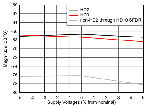
F_{IN} = 347 MHz
