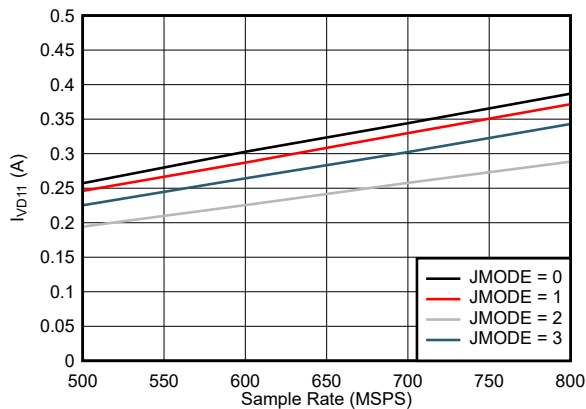
Figure 7-77. Quad Channel, I_{VD11} vs F_S for JMODES 0 - 3 Independent of Power Mode
