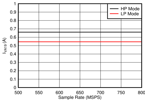
Figure 7-75. Quad Channel, I_{VA19} vs F_S Independent of JMODE
