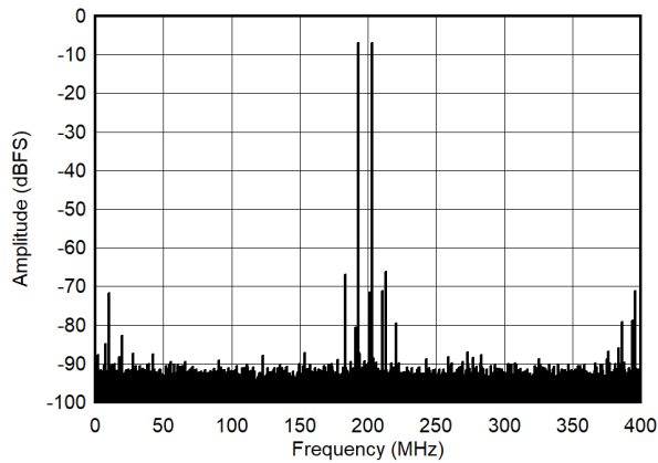
Figure 7-53. Single Tone FFT at 1798 MHz
