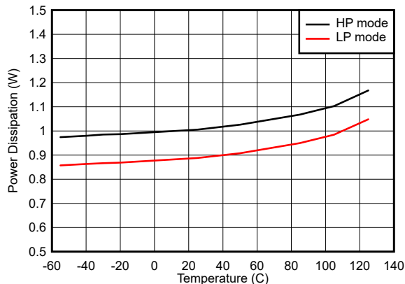
Figure 7-115. Single Channel, Power Dissipation vs Temperature
