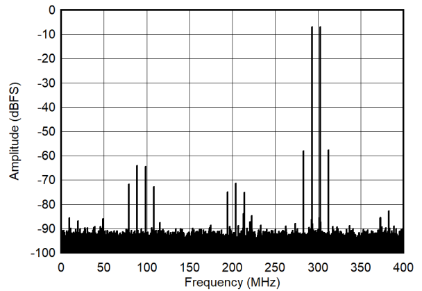
Figure 7-54. Single Tone FFT at 2698 MHz
