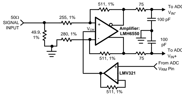
Figure 41. Differential Drive Circuit of Figure 40
