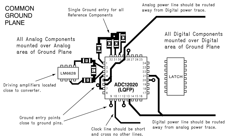
Figure 43. Example of a Suitable Layout
