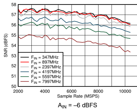
Figure 6-30. DES Mode: SNR vs Sample Rate and Input Frequency A_{IN} = -6\text{ dBFS}
