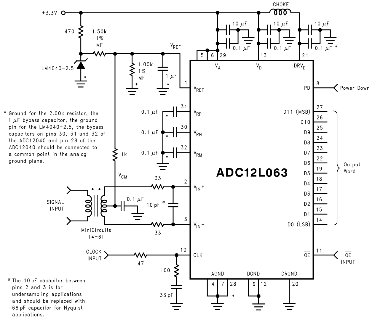
Figure 35. Driving the Signal Inputs with a Transforme
