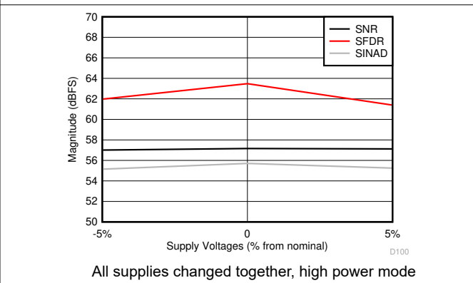
Figure 7-60. SNR, SFDR and SINAD vs Supply Voltage
