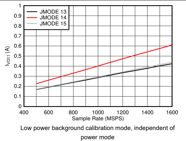
Figure 7-88. Quad Channel, I_{VD11} vs F_S and JMODE 13 - 15
