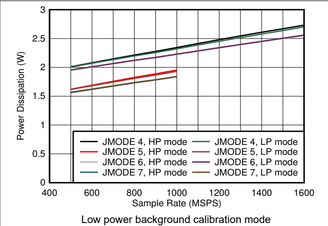
Figure 7-80. Quad Channel, Power Dissipation vs F_S and JMODE 4 - 7
