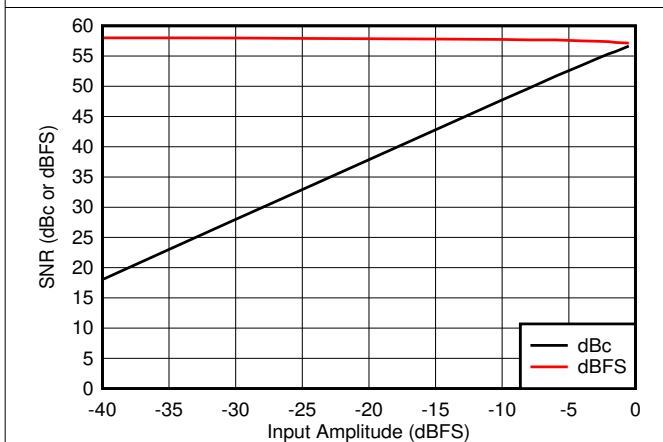
Figure 7-33. SNR vs A_{IN}
