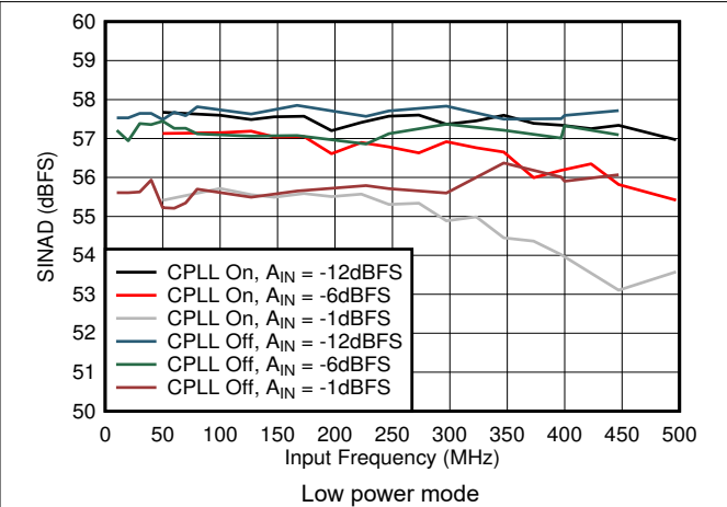
Figure 7-56. SINAD vs A_{IN} and C-PLL
