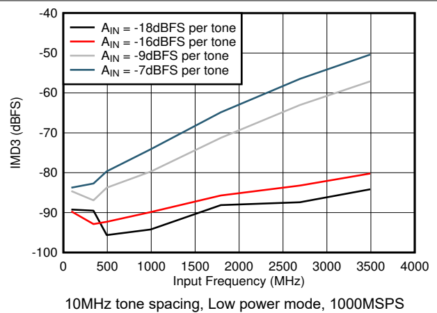
Figure 7-76. IMD3 vs F_{IN}
