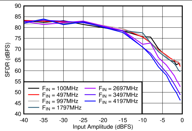
Figure 7-32. SFDR vs A_{IN}
