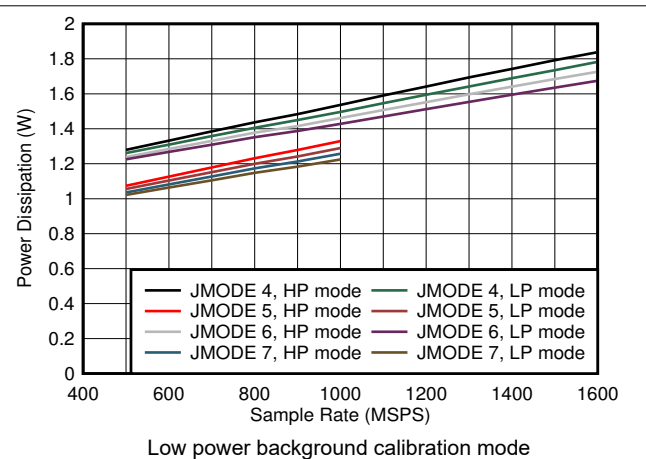
Figure 7-90. Dual Channel, Power Dissipation vs F_S and JMODE 4 - 7
