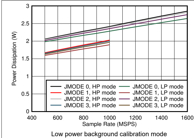
Figure 7-79. Quad Channel, Power Dissipation vs F_S and JMODES 0 - 3
