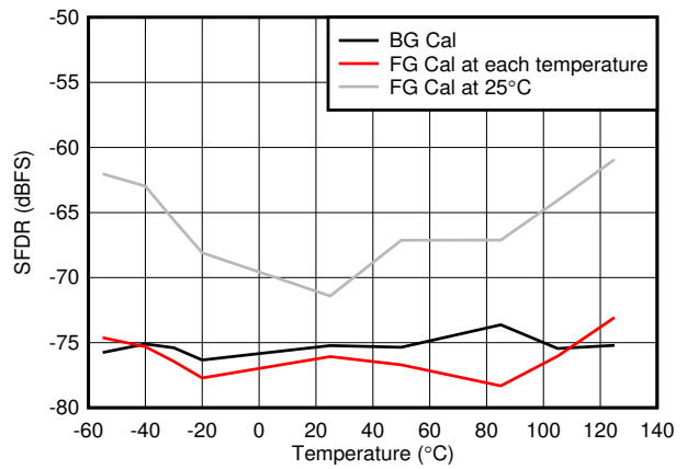
Figure 7-68. Worst Spur vs Temperature
