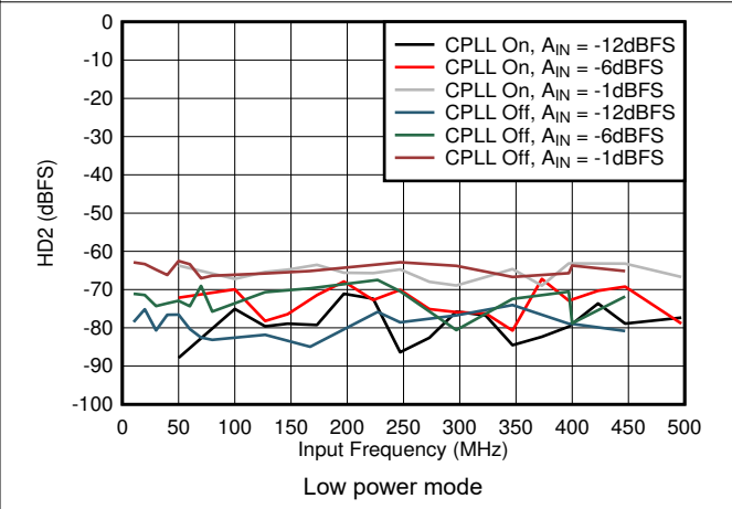
Figure 7-58. HD2 vs A_{IN} and C-PLL
