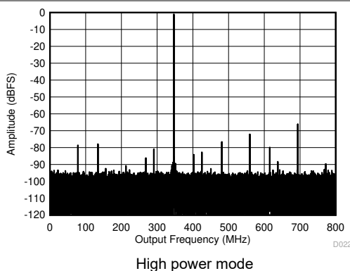
Figure 7-4. Single Tone FFT at 347 MHz and -1 dBFS
