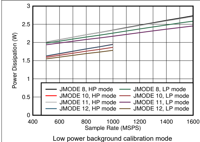
Figure 7-81. Quad Channel, Power Dissipation vs F_S and JMODE 8 - 12
