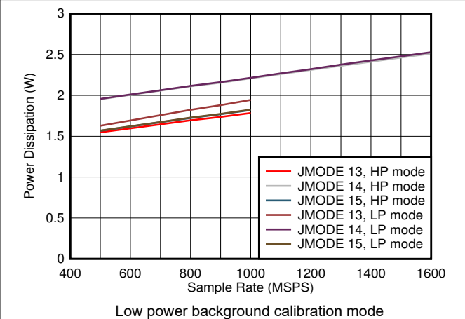
Figure 7-82. Quad Channel, Power Dissipation vs F_S and JMODE 13 - 15
