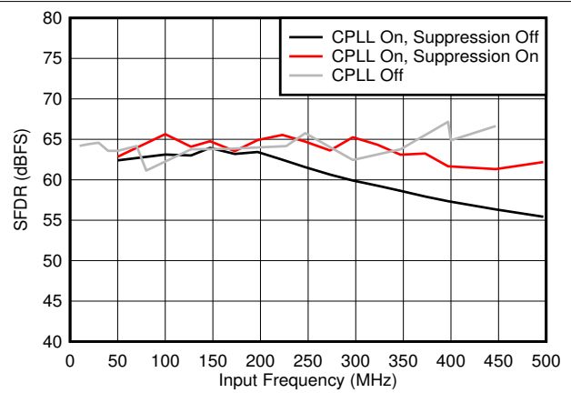
Figure 7-44. SFDR vs F_{IN} and C-PLL modes
