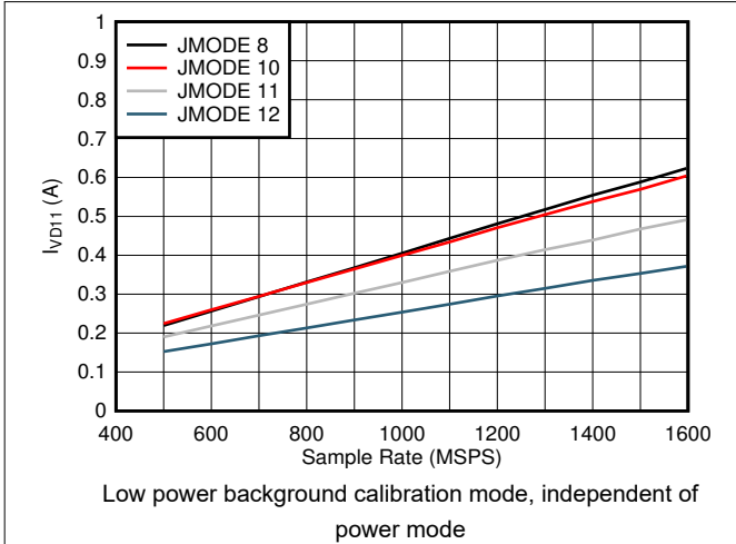
Figure 7-87. Quad Channel, I_{VD11} vs F_S and JMODE 8 - 12
