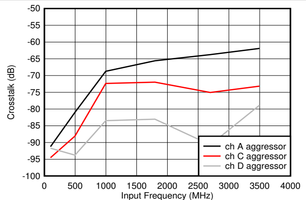
Figure 7-78. Crosstalk to Channel B vs F_{IN}
