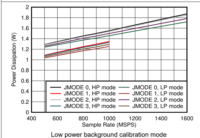
Figure 7-89. Dual Channel, Power Dissipation vs F_S and JMODE 0 - 3
