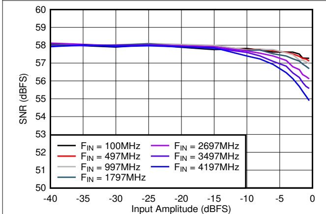
Figure 7-33. SNR vs A_{IN}
