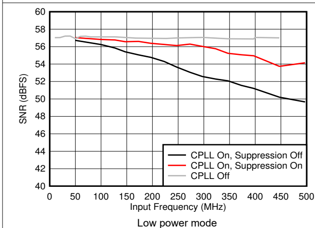
Figure 7-45. SNR vs F_{IN} and C-PLL modes
