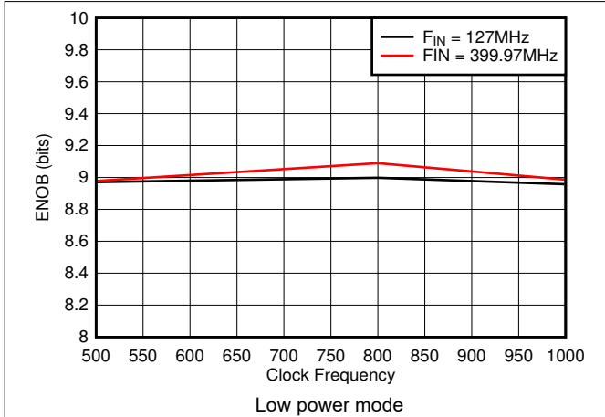
Figure 7-31. ENOB vs Sample Rate
