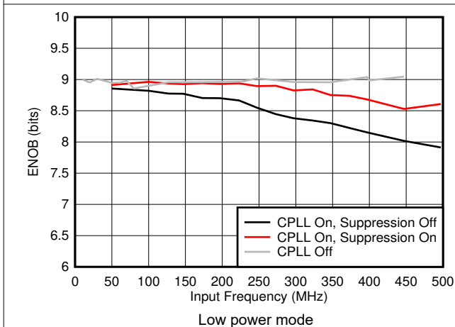
Figure 7-47. ENOB vs F_{IN} and C-PLL modes
