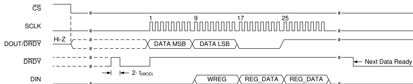
Figure 8-30. Example of Reading Data While Simultaneously Sending a \text{WREG} Command
