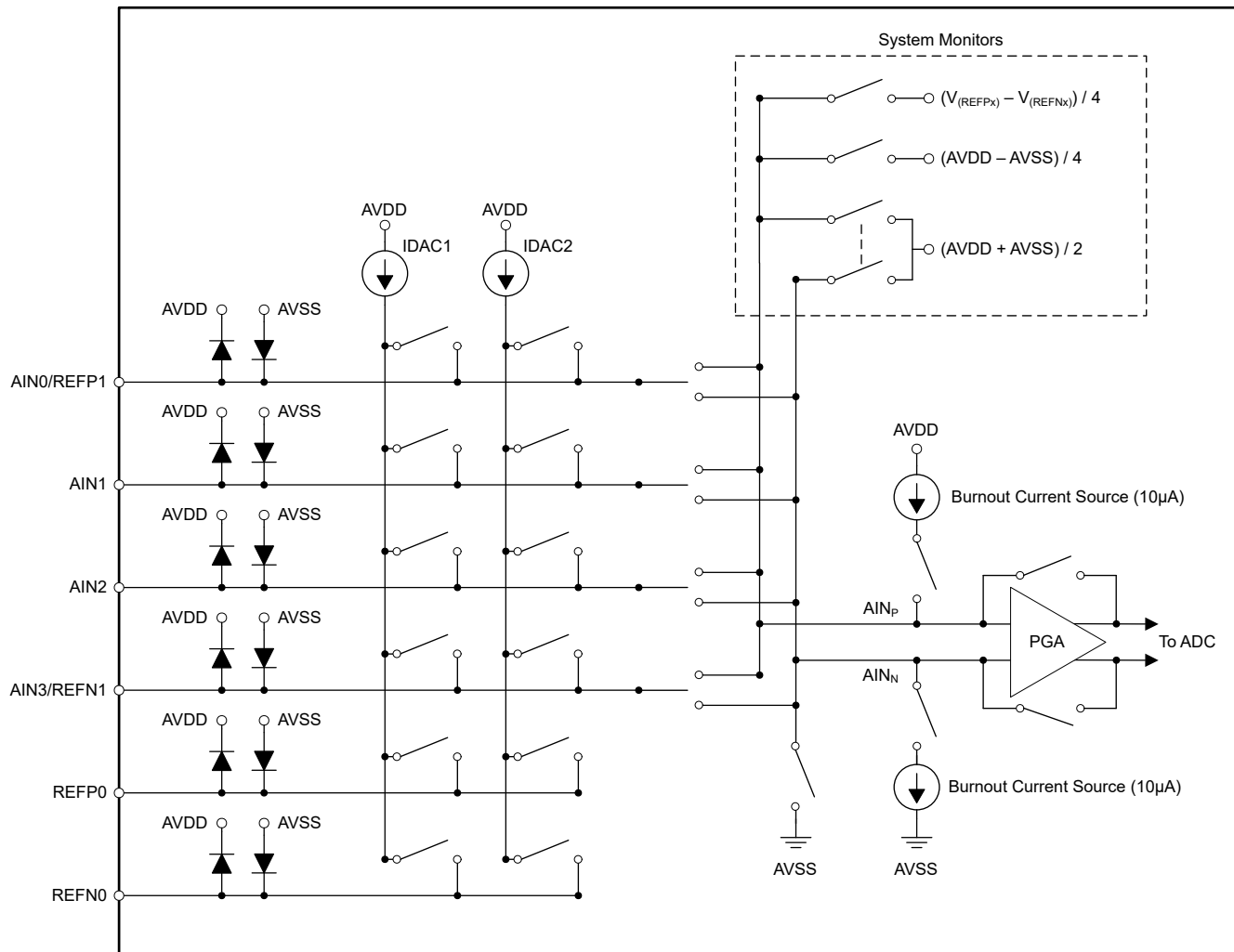
Figure 8-1. Analog Input Multiplexer
