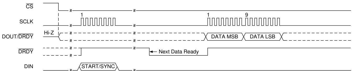
Figure 8-27. Single-Shot Conversion Mode ( \text{DRDYM} = 0\text{b} )
