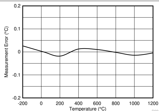
Figure 9-5. Temperature Measurement Error vs T_{\text{TC}}
