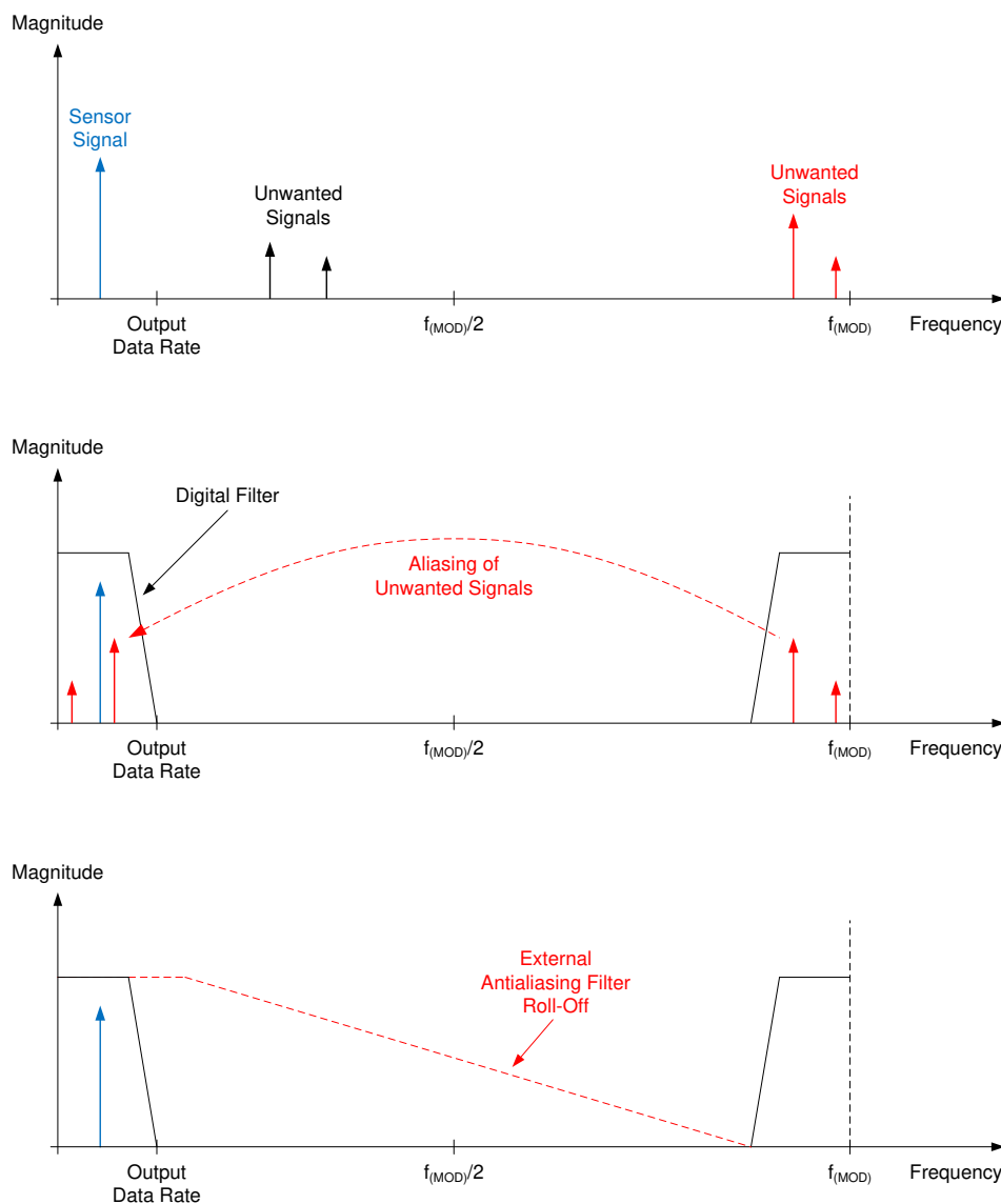
Figure 9-2. Effect of Aliasing
