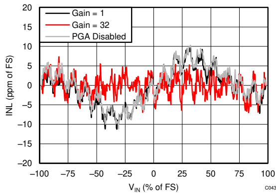
Figure 6-9. Integral Nonlinearity vs Differential Input Signal
