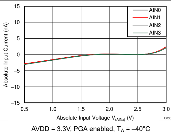
Figure 6-15. Absolute Input Current vs Absolute Input Voltage
