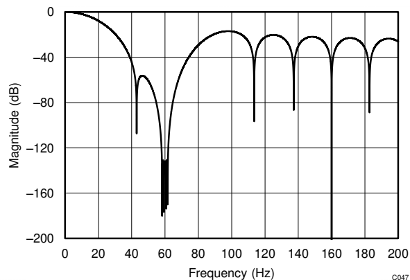
Figure 8-13. Filter Response (DR = 20SPS)
