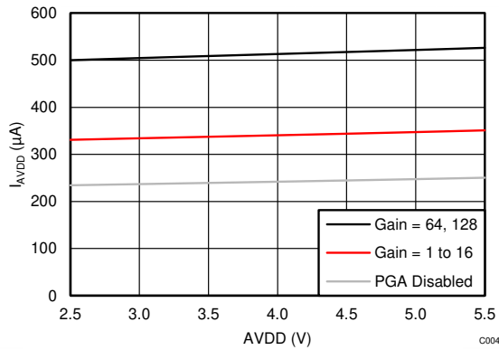
Figure 6-33. I_{AVDD} vs AVDD
