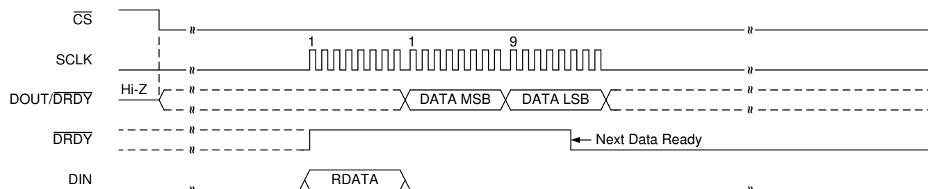
Figure 8-28. State of \overline{\text{DRDY}} When a New Conversion Finishes During an \text{RDATA} Command
