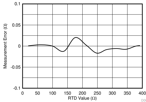
Figure 9-9. Resistance Measurement Error vs R_{\text{RTD}}
