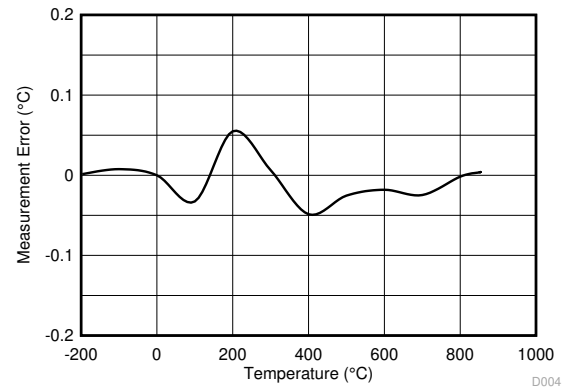
Figure 9-10. Temperature Measurement Error vs T_{\text{RTD}}
