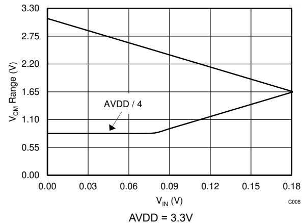
Figure 8-5. Common-Mode Voltage Limits
