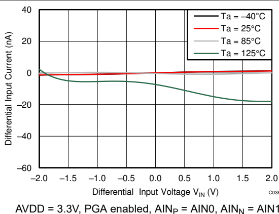
Figure 6-19. Differential Input Current vs Differential Input Voltage
