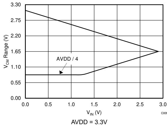
Figure 8-4. Common-Mode Voltage Limits
