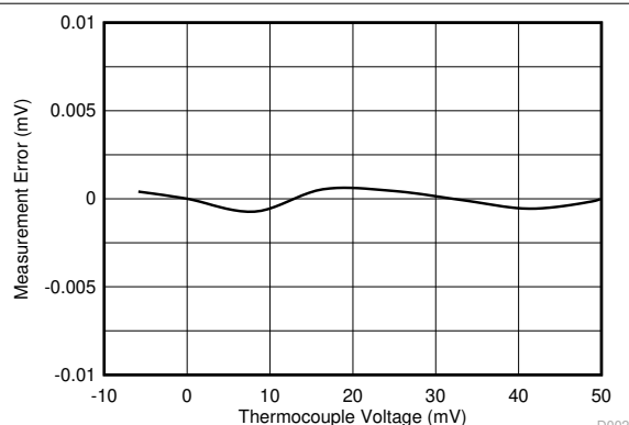
Figure 9-4. Voltage Measurement Error vs V_{\text{TC}}
