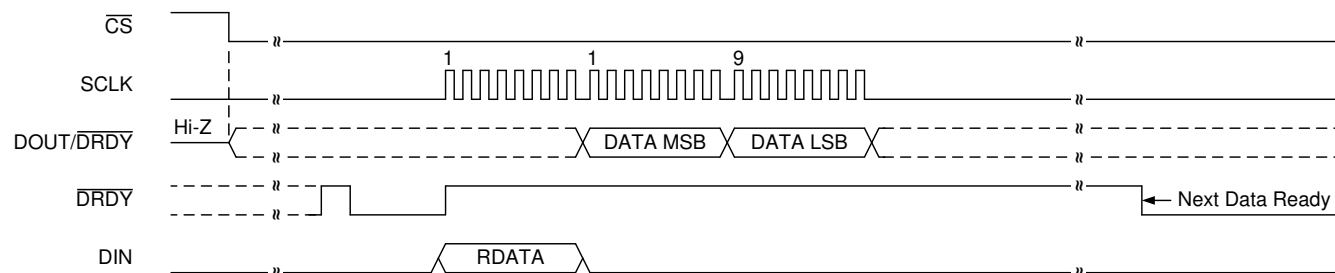
Figure 8-29. State of \overline{\text{DRDY}} When the Most Recent Conversion Result is Read During an \text{RDATA} Command
