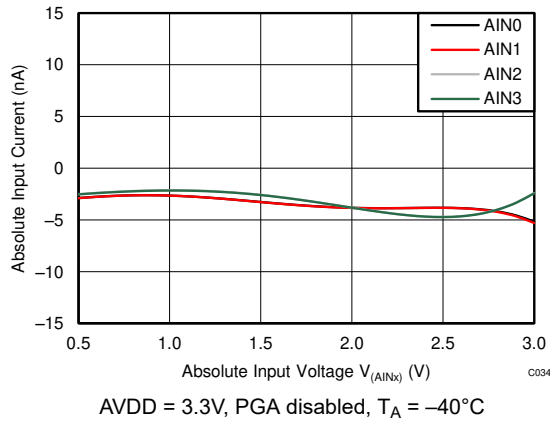
Figure 6-21. Absolute Input Current vs Absolute Input Voltage
