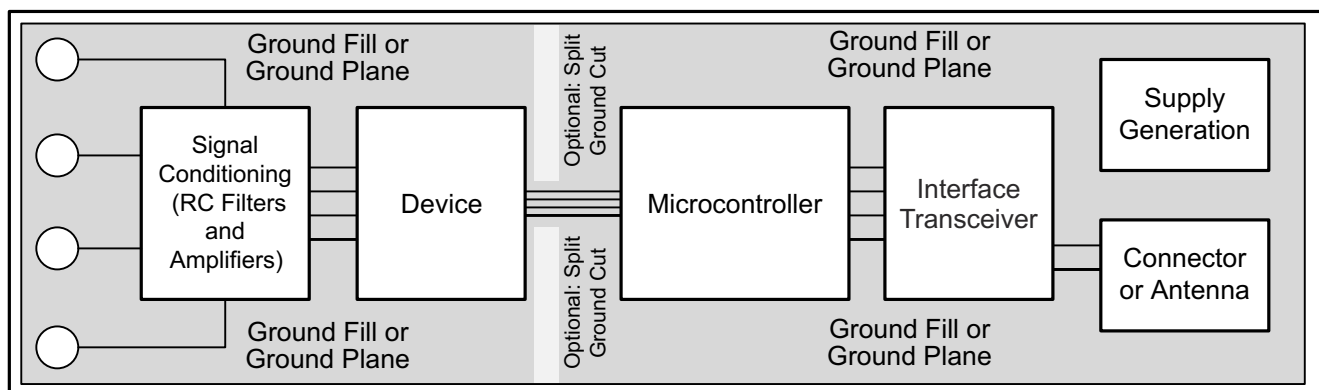
Figure 9-15. System Component Placement
